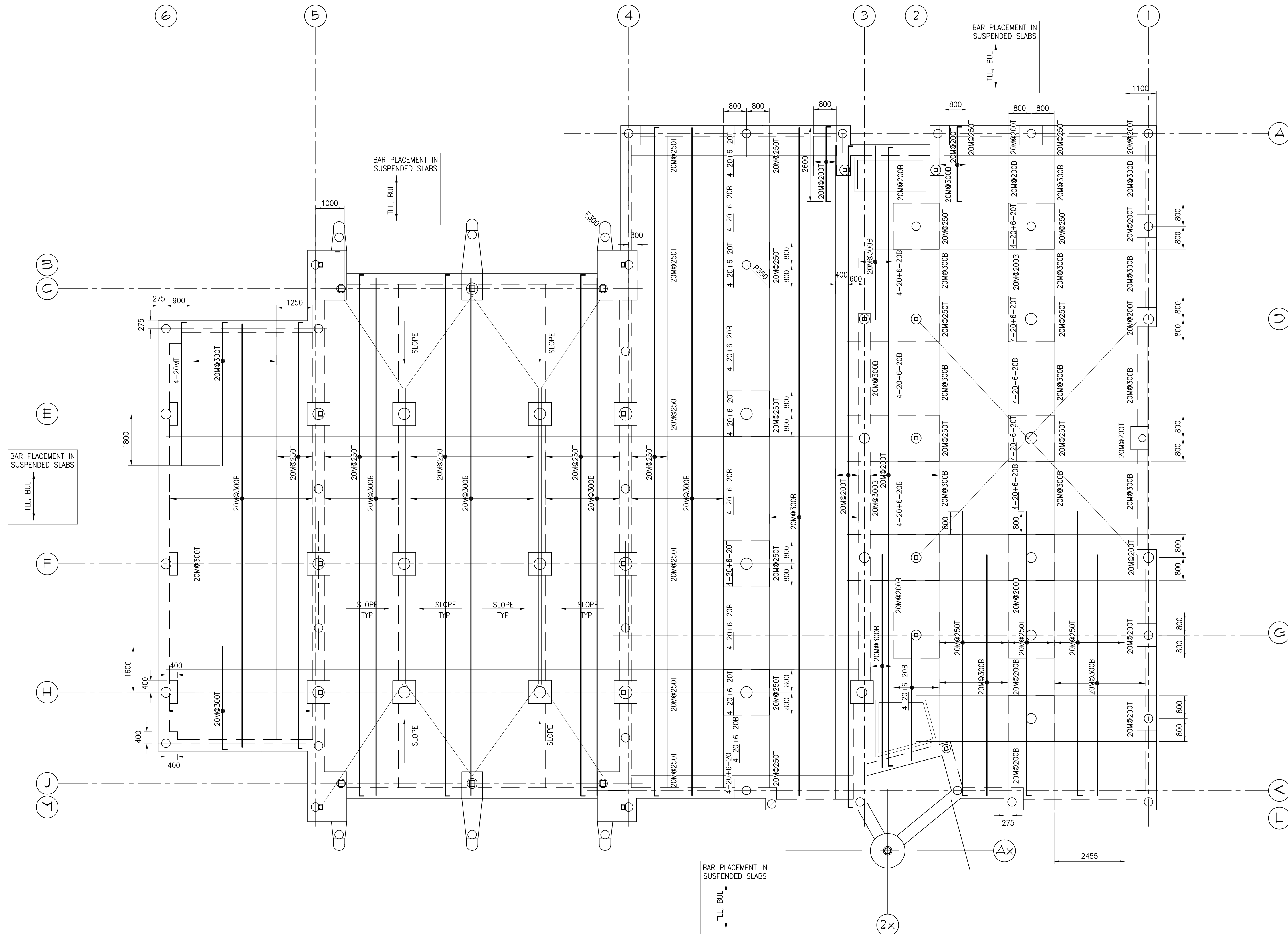
FLOOR SLAB FRONT REAR DIRECTION REINFORCING SCALE: 1:75
