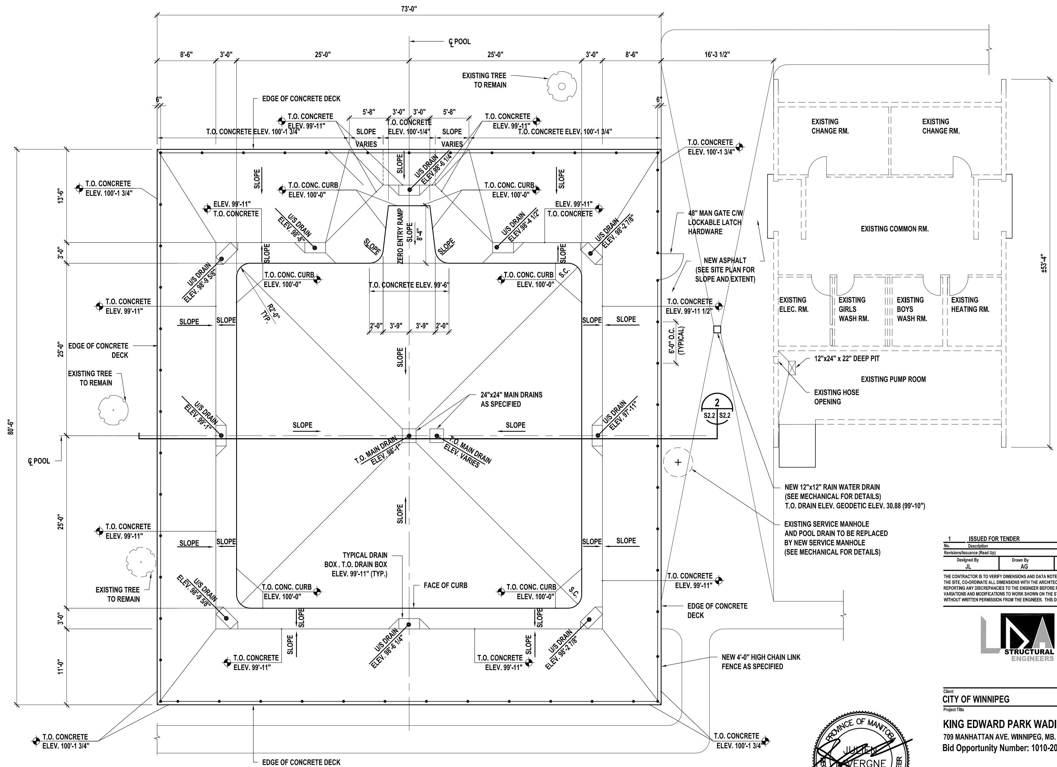
NEW POOL PLAN Scale= 1/8"=1'-0"
