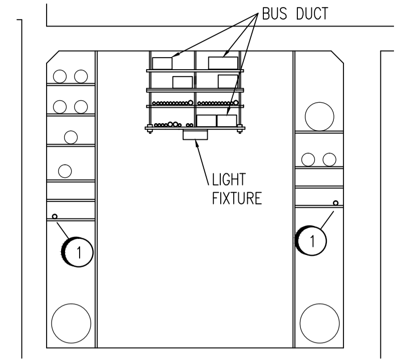
GALLERY 3 SCALE 1:50
