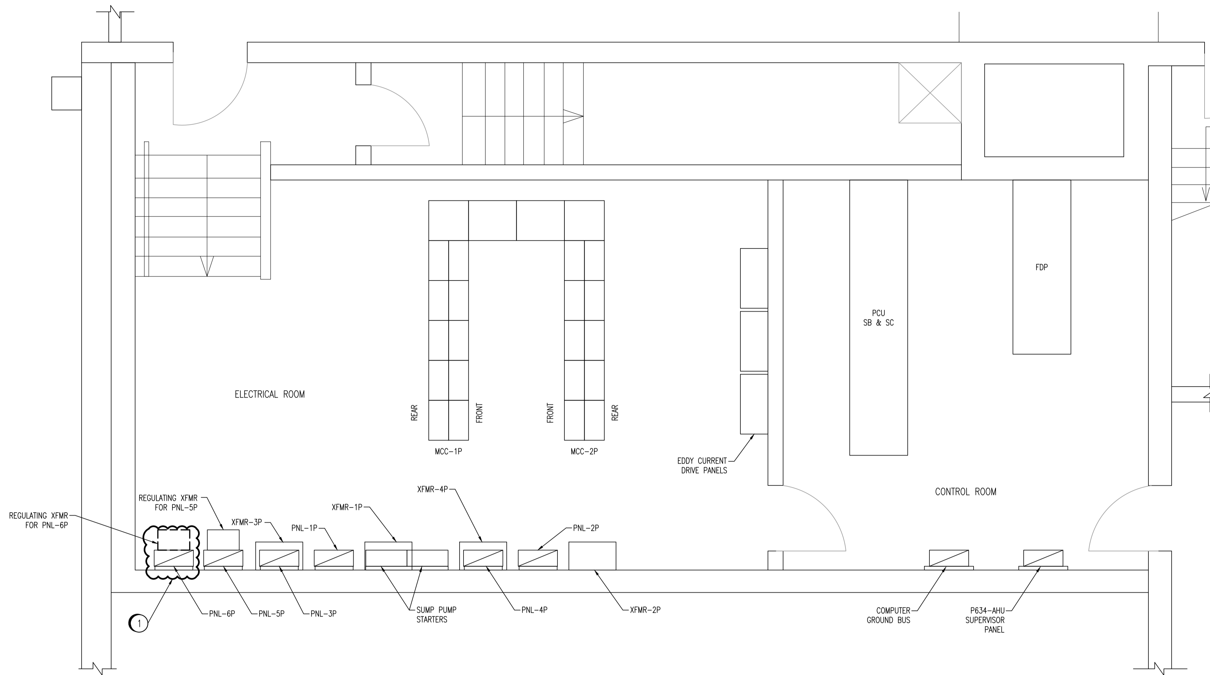
PRIMARY CLARIFIER ELECTRICAL AND CONTROL ROOMS 1:30
