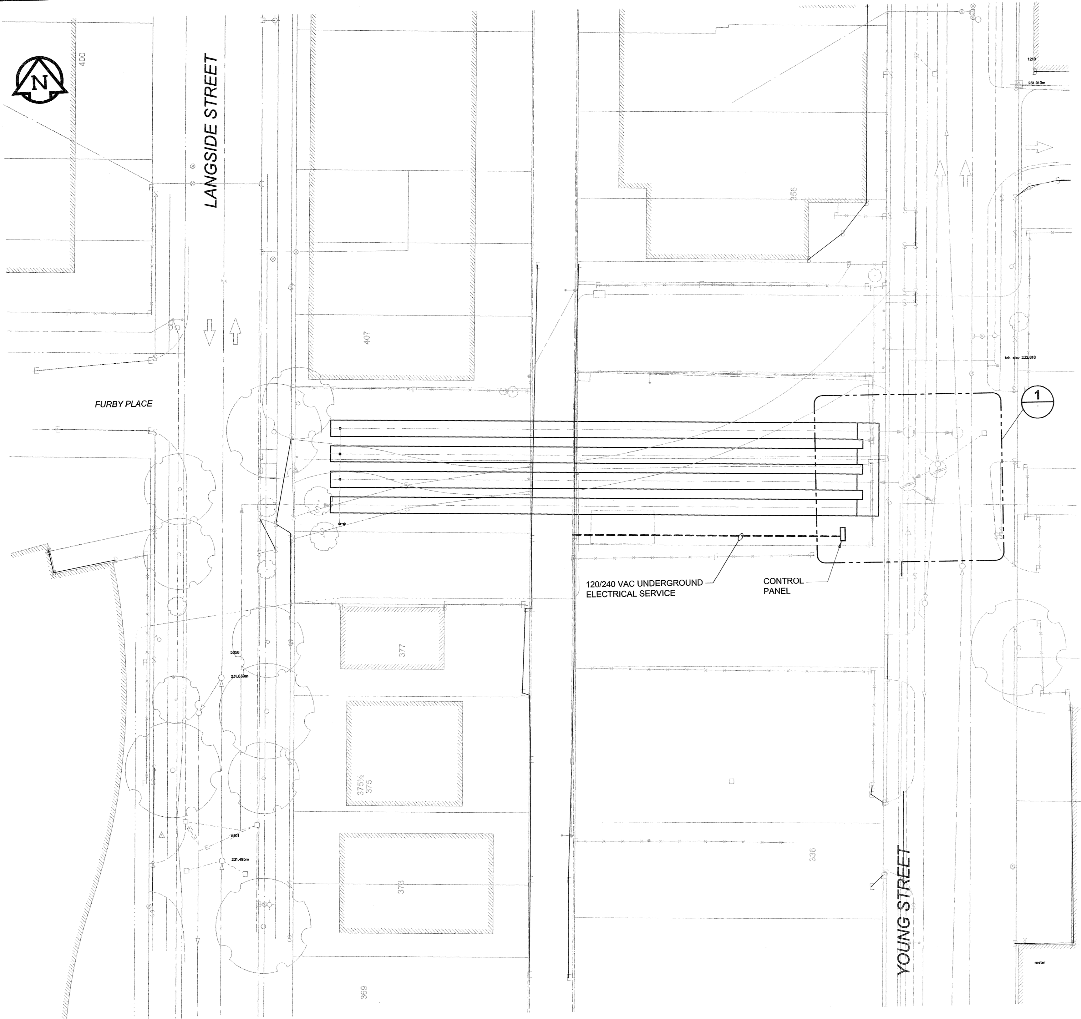
SITE PLAN 0 2.5 5 7.5 m SCALE 1:250
