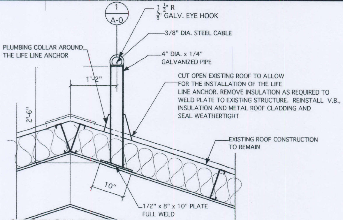
1 SECTION DETAIL S-7 SCALE: 3/4" = 1'-0"
