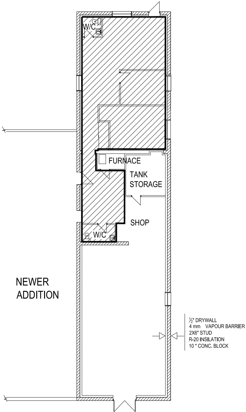
FLOOR PLAN-825 TACHE
