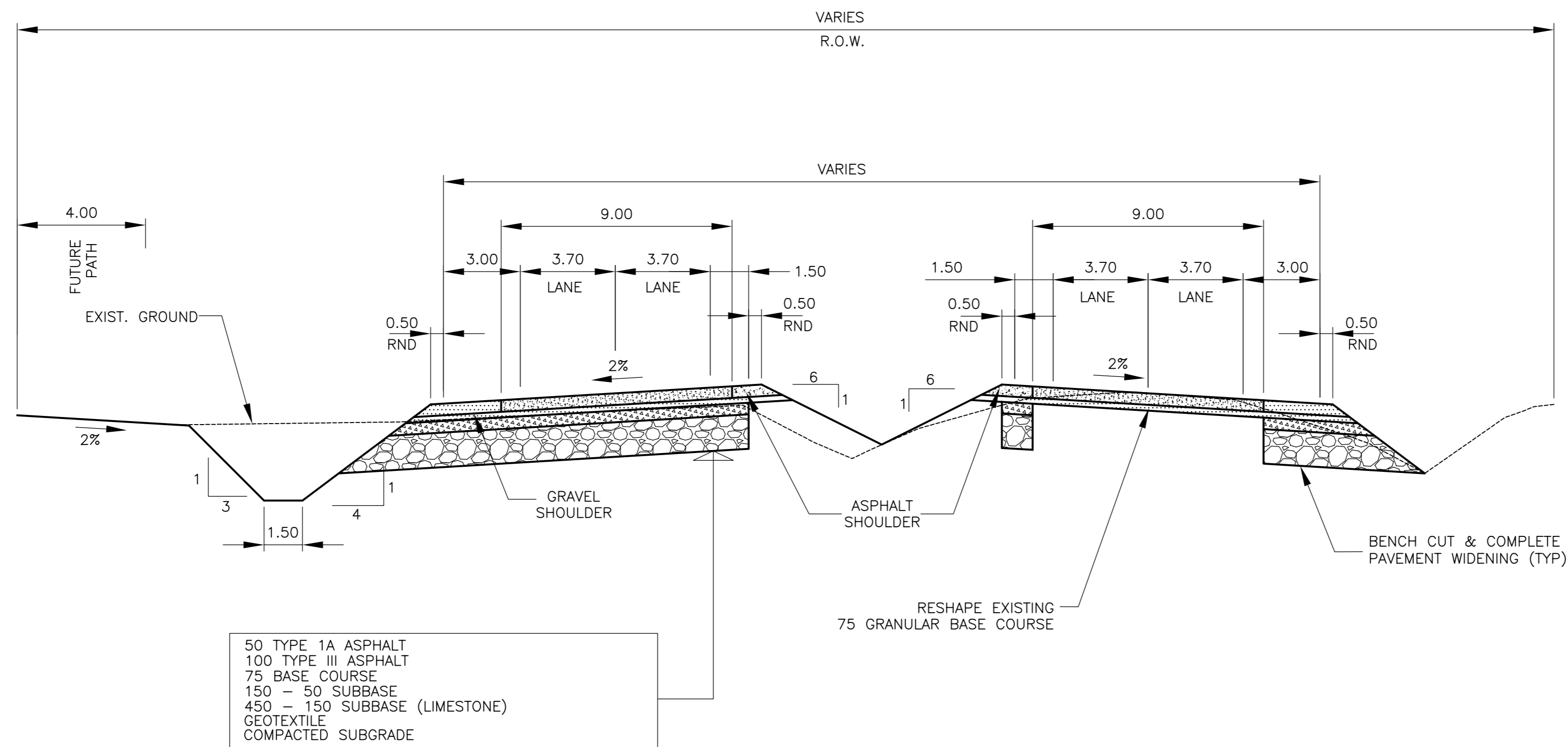
5 WAVERLEY STREET TYPICAL SECTION HORZ. 1:150 VERT. 1:50
