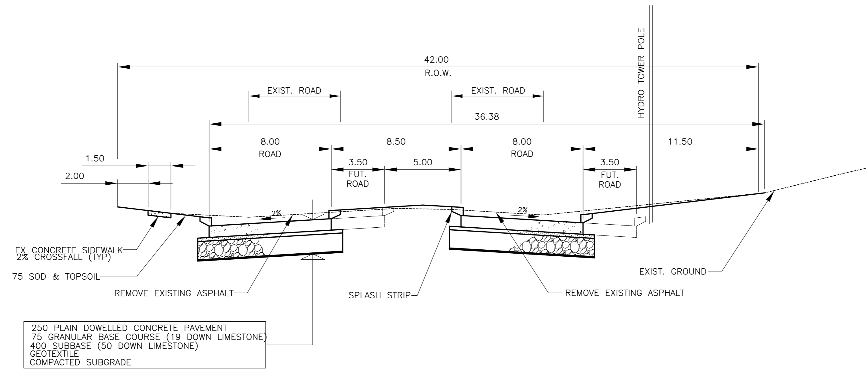
1 WAYERLEY STREET TYPICAL SECTION HORZ. 1:150 VERT. 1:50
