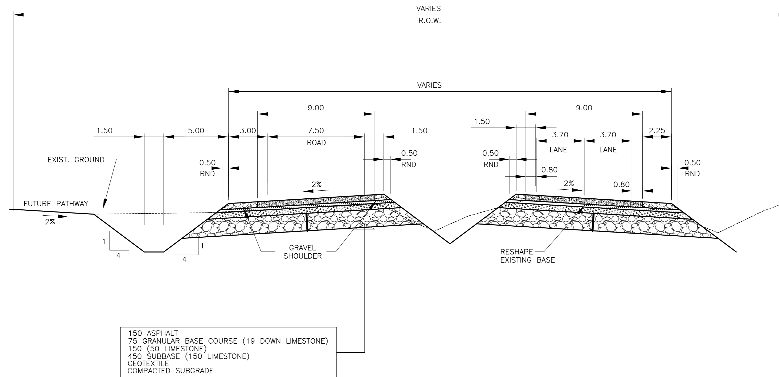
5 WAYERLEY STREET TYPICAL SECTION 10 | 18 HORZ. 1:150 VERT. 1:50
