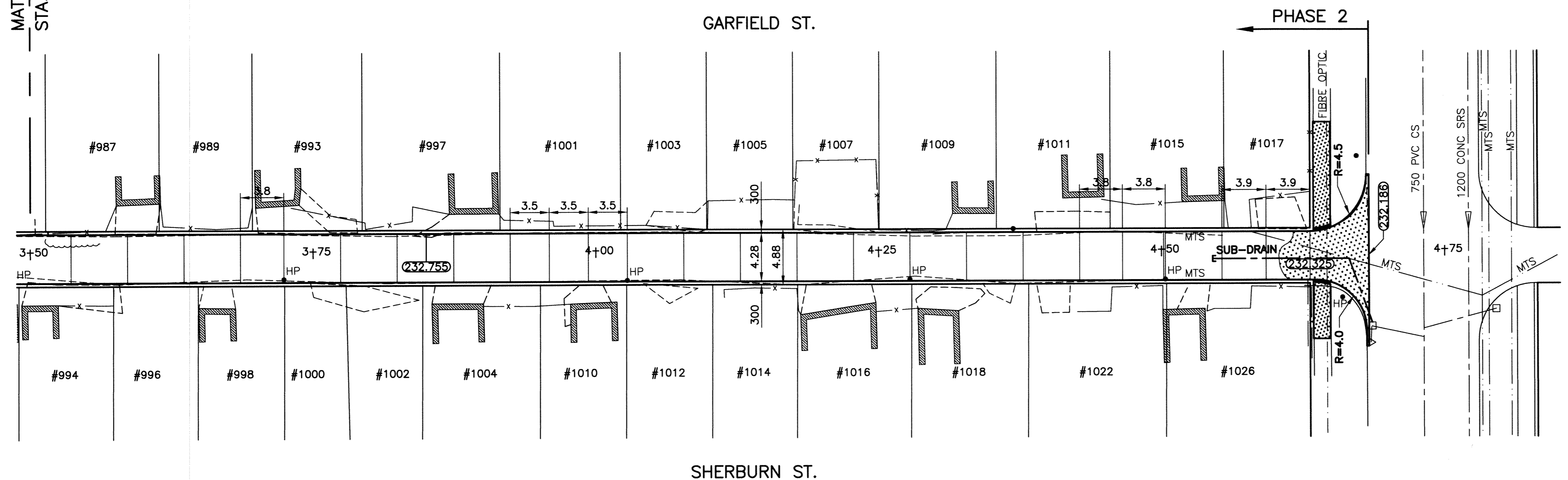
ALLEY PAVEMENT PLAN SCALE: 1:250 HOR
