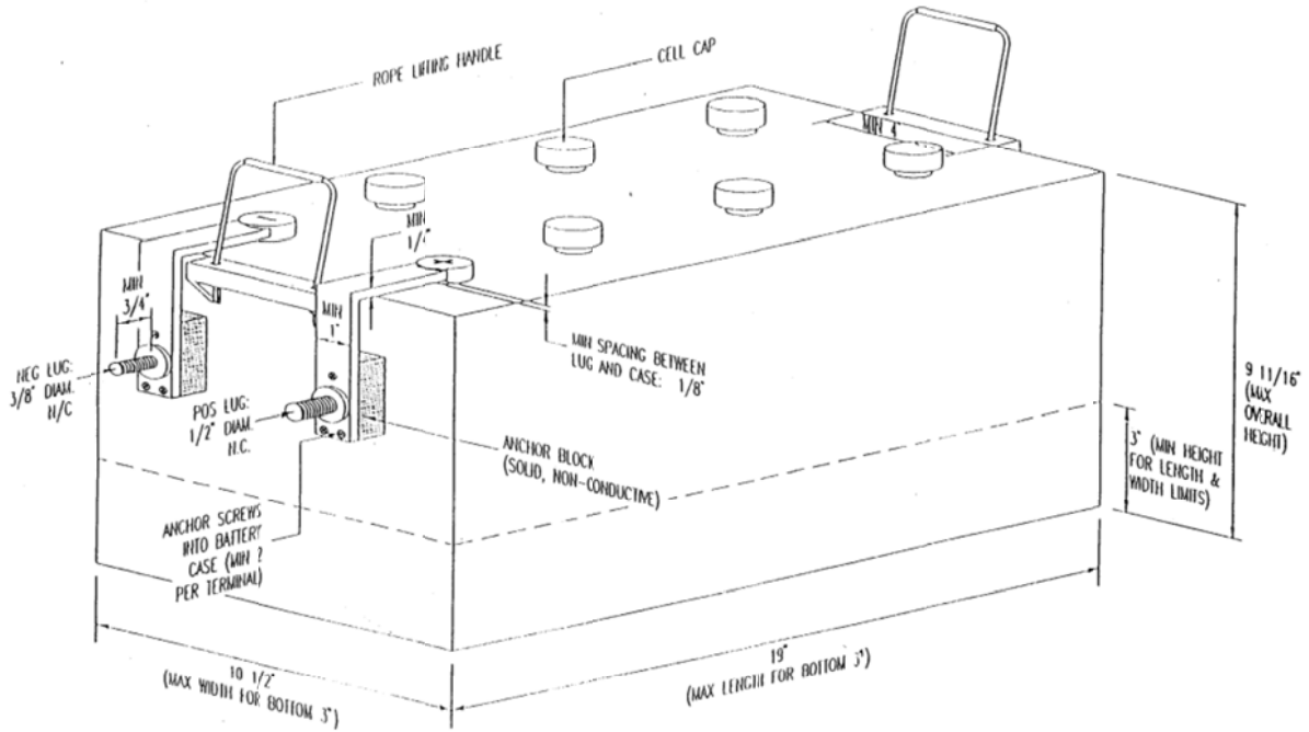
BUS BATTERY WITH DROP TERMINALS - Dimensional Specifications -
