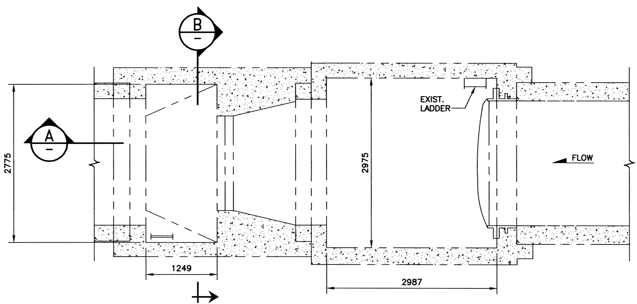
PLAN - EL. 223.26
