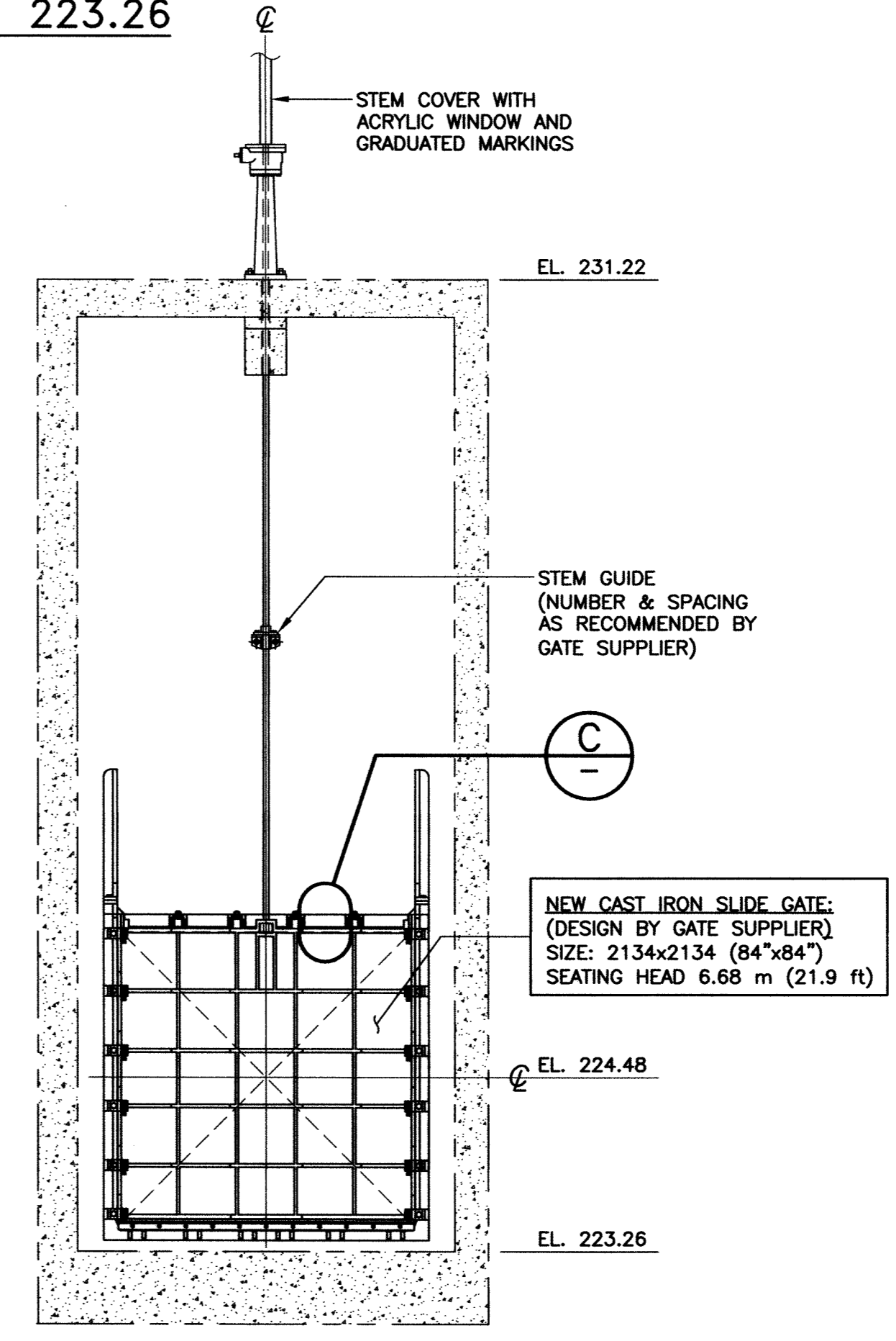
(NEW SLIDE GATE) B2 SECTION SCALE: 1:40
