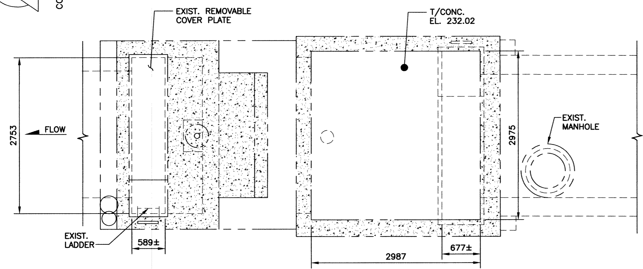
PLAN - EL. 231.22
