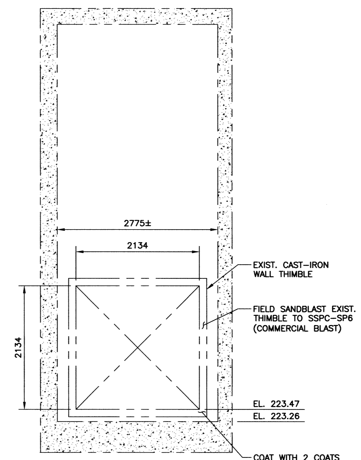
(EXIST. OPENING) B1 SECTION SCALE: 1:40
