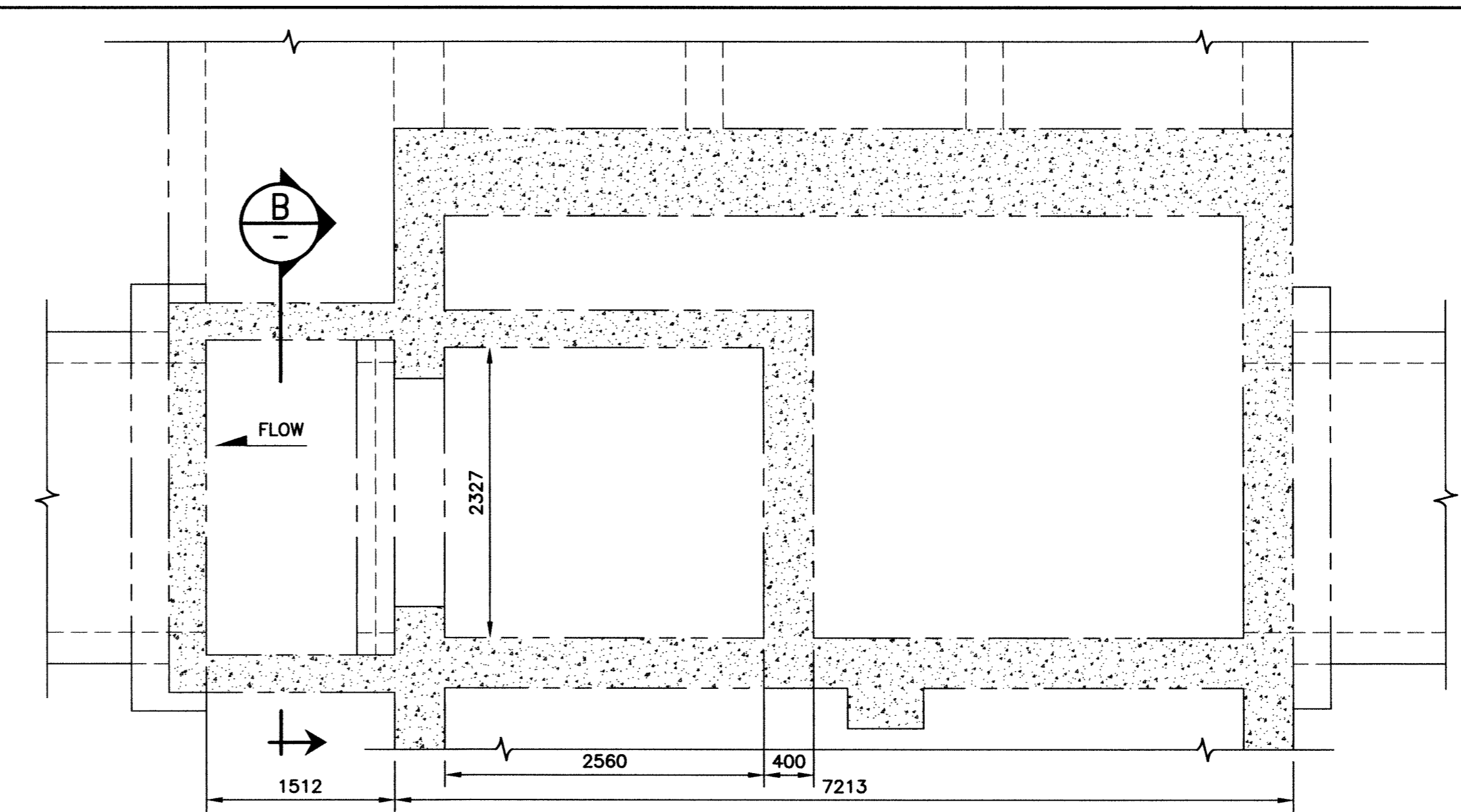
PLAN - EL. 222.76 SCALE: 1:40
