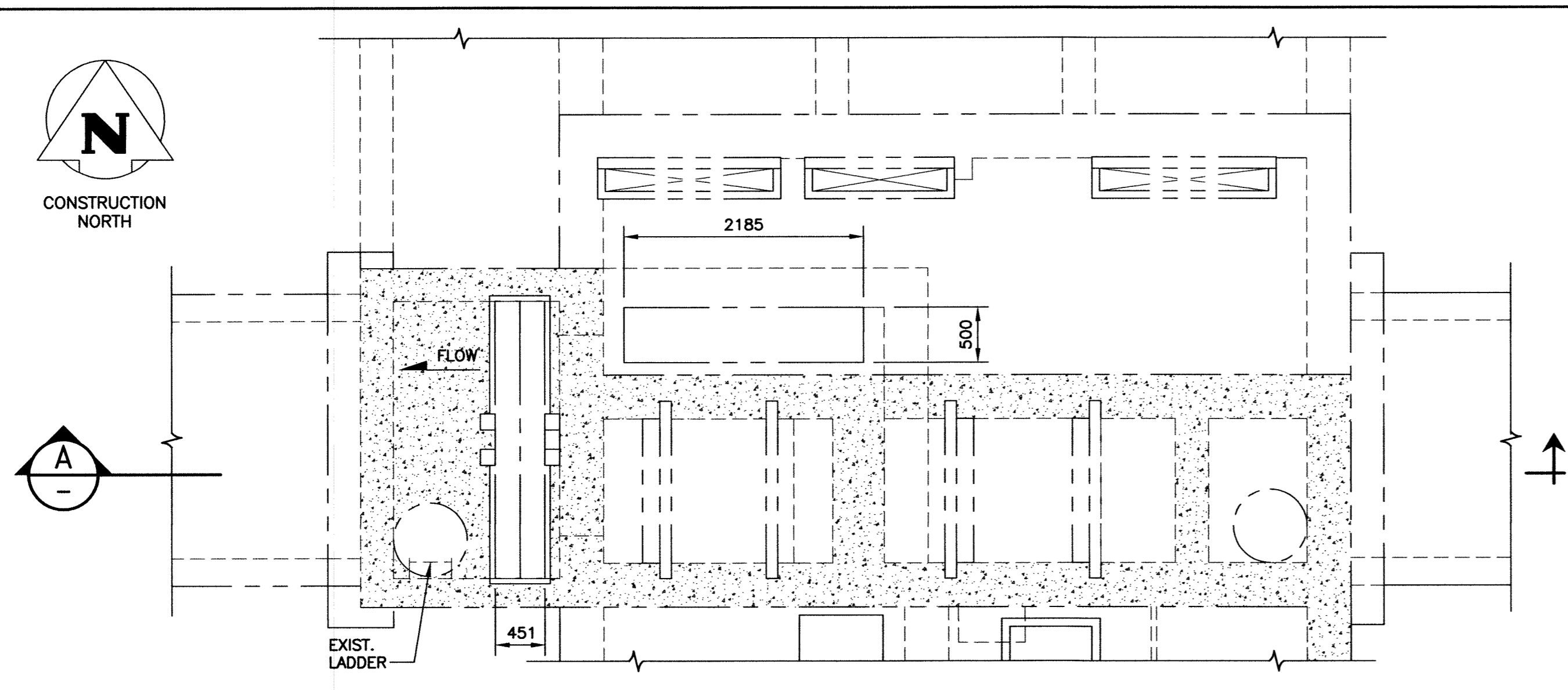
PLAN - EL. 231.88 SCALE: 1:40
