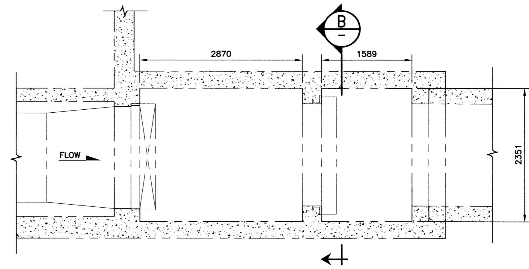
PLAN - EL. 222.55 SCALE: 1:40
