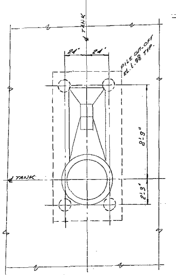
DETAIL OF TANK CENTRE SCALE 1/4" = 1'-0"
