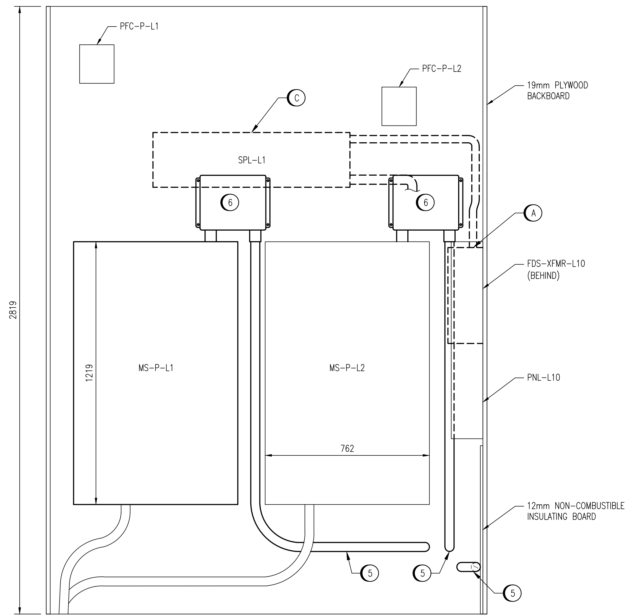
ELEVATION DETAIL - EAST WALL SCALE: 1 : 10
