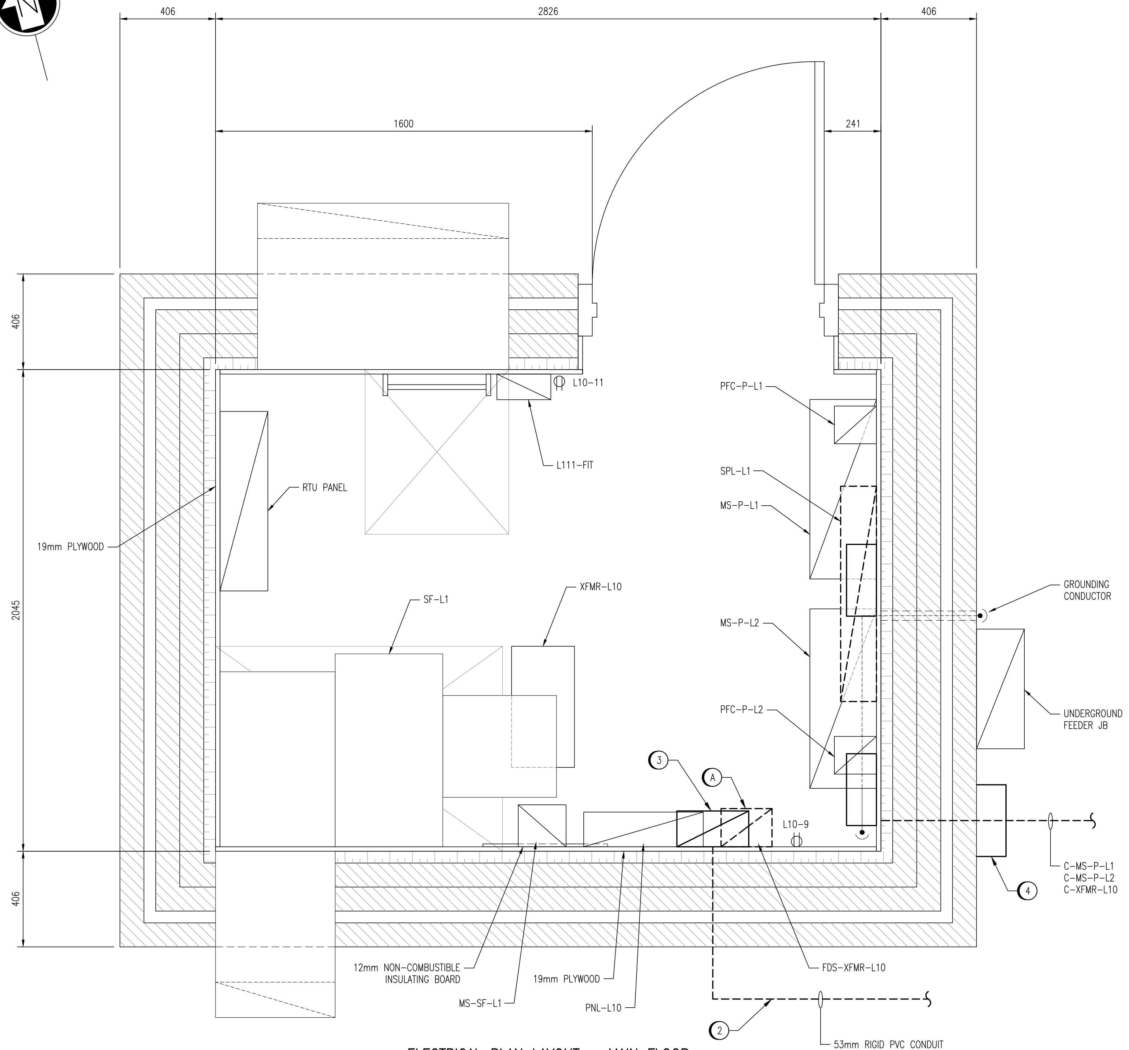
ELECTRICAL PLAN LAYOUT - MAIN FLOOR SCALE: 1 : 10
