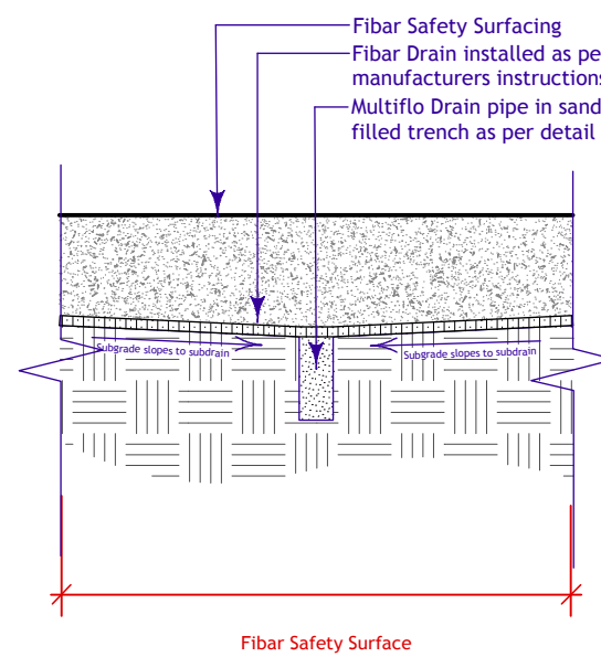
Section A
