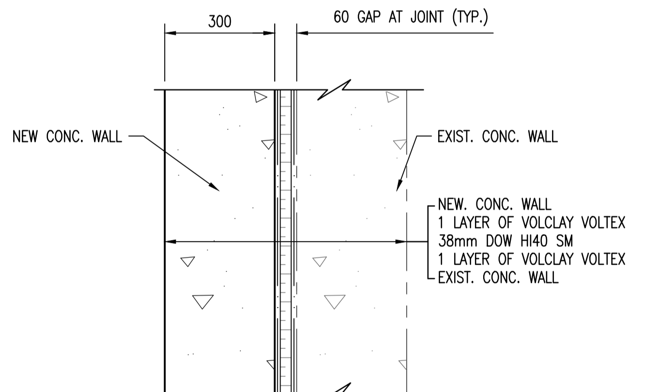
JOINT AT COMMON WALL SCALE: 1 : 10
