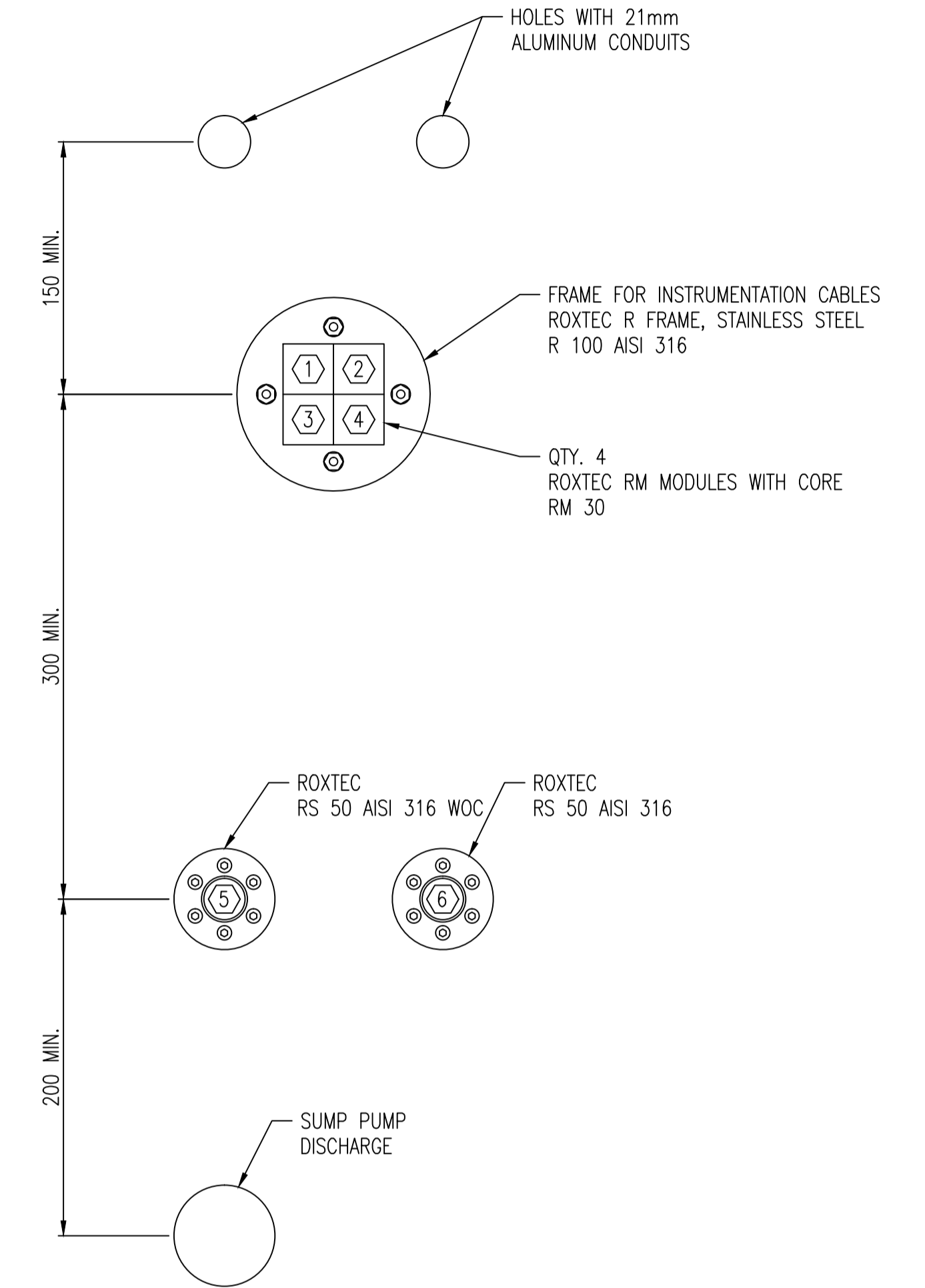
1 - DETAIL : CABLE SEAL INSTALLATION SCALE: 1 : 3
