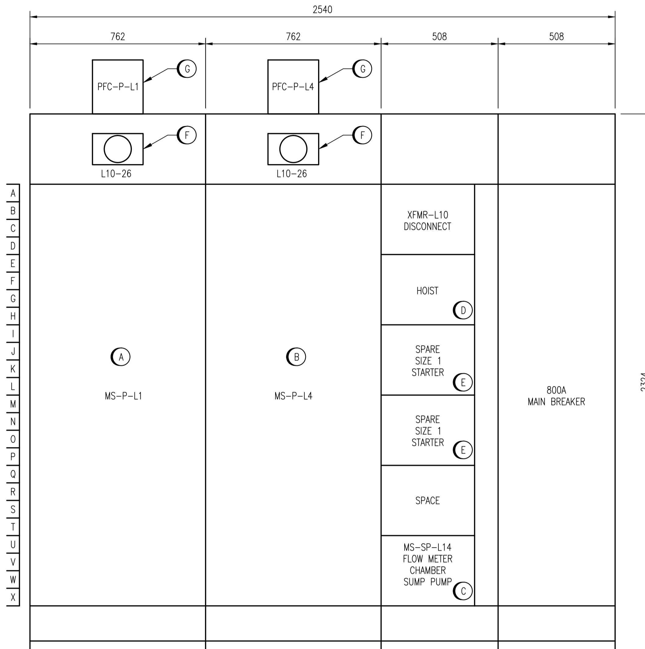
MCC-L2 - FRONT ELEVATION SCALE: 1 : 10
