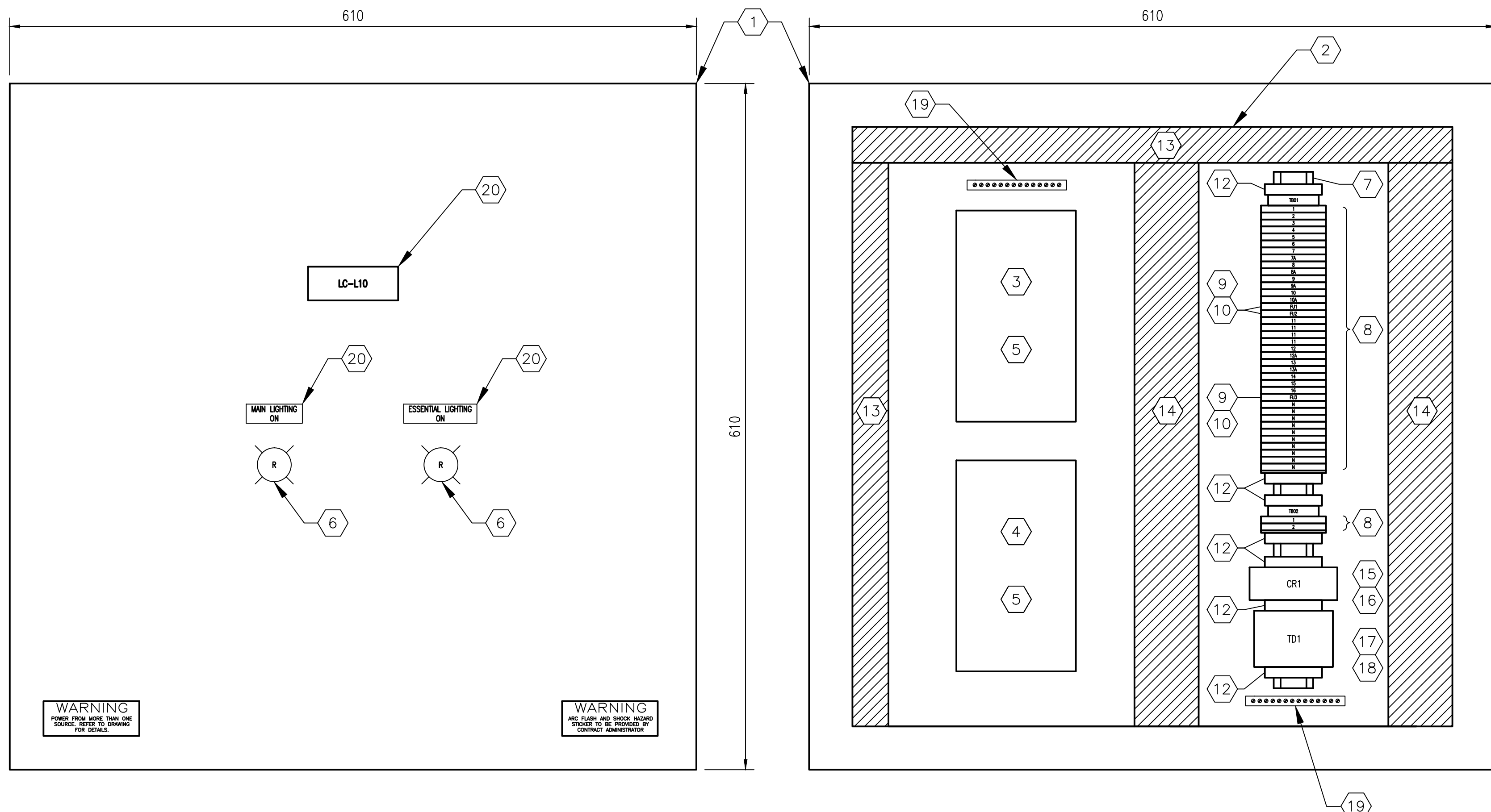
EXTERIOR PANEL VIEW SCALE: 1:3
