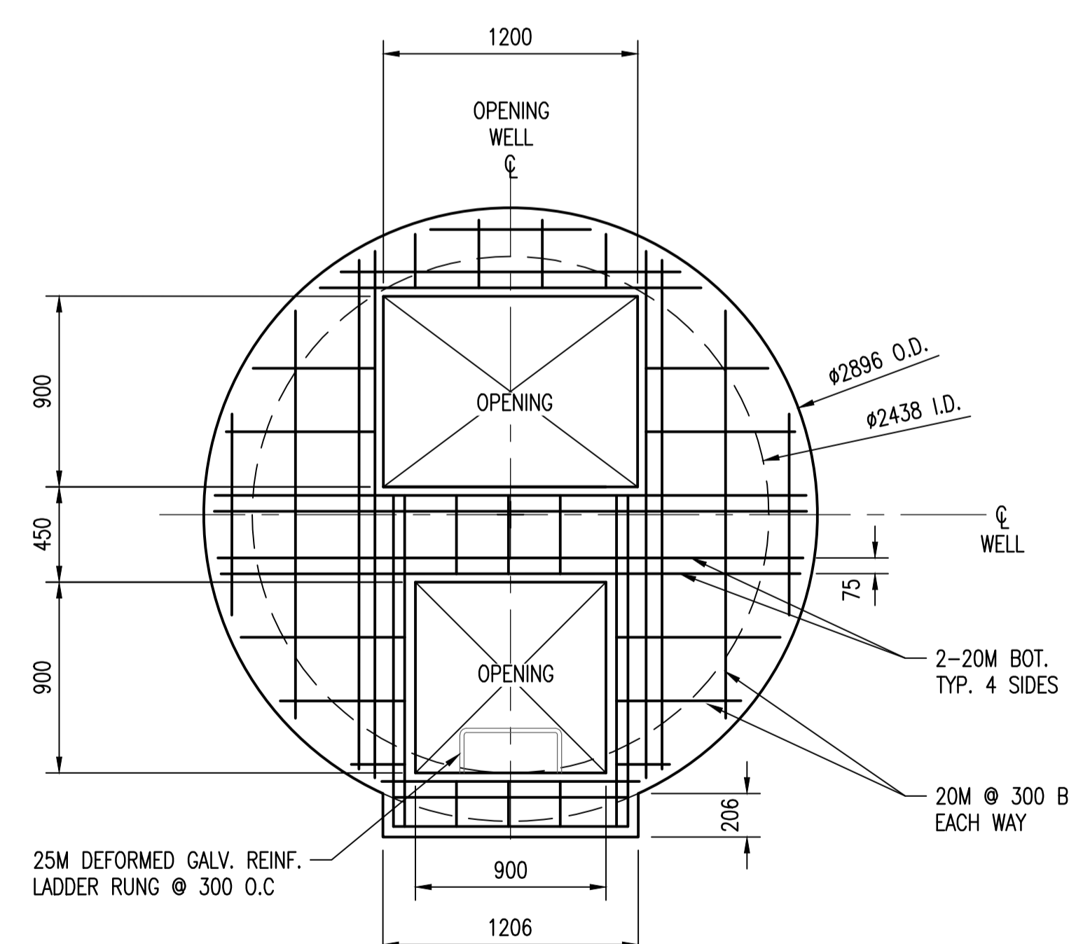
PLAN-TOP SLAB ELEVATION 230.732m SCALE: 1 : 25
