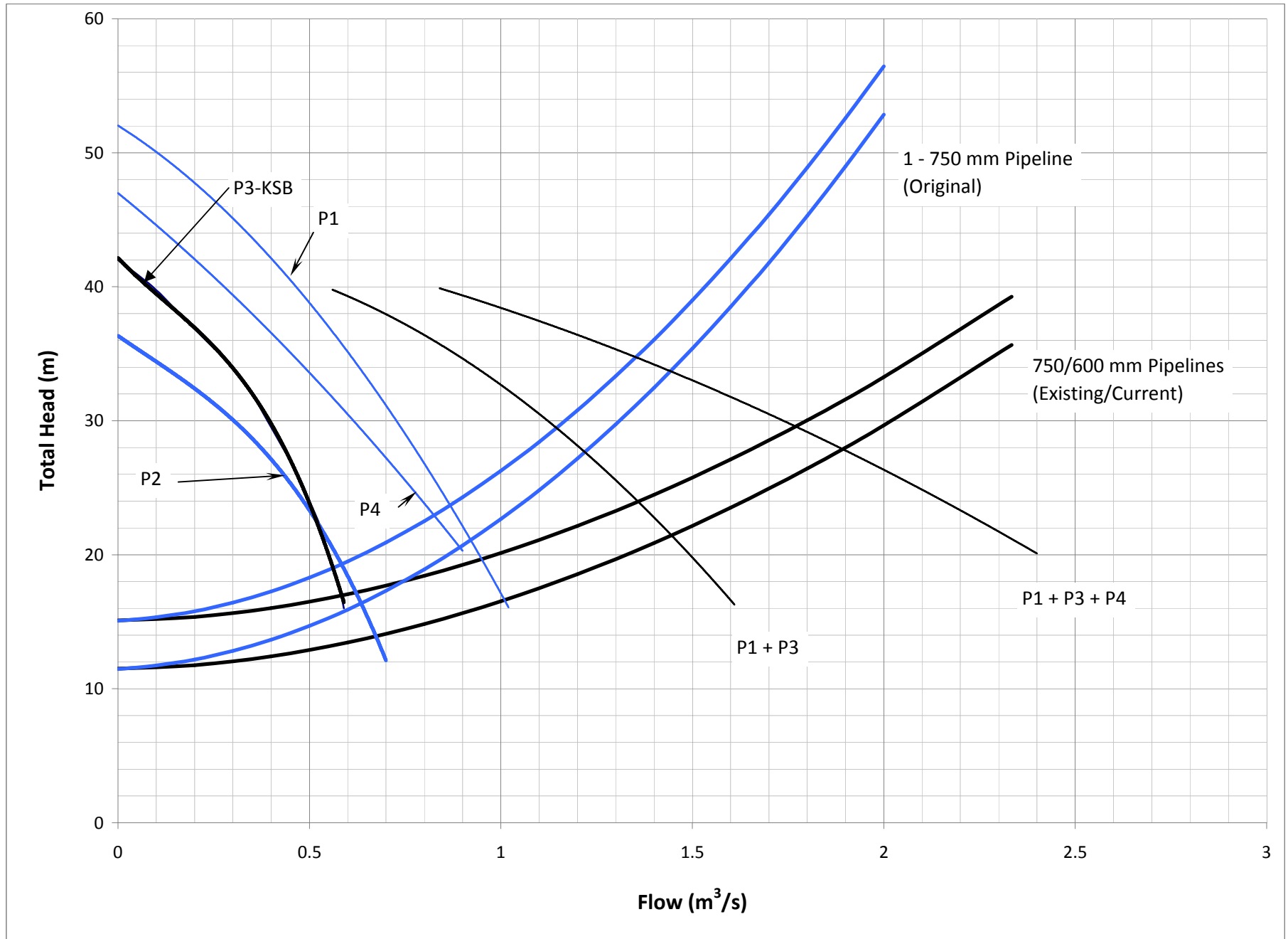
FIGURE 2.1 Perimeter Road Pumping Station - System Curve
