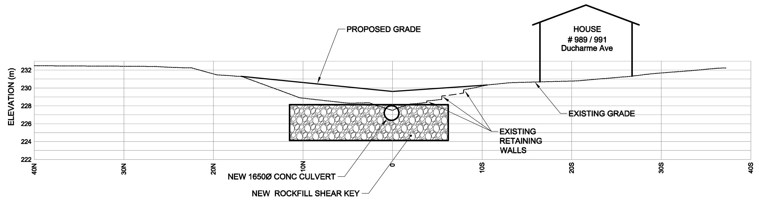
SECTION 0+993 0 2.5 5 7.5 m SCALE 1:250
