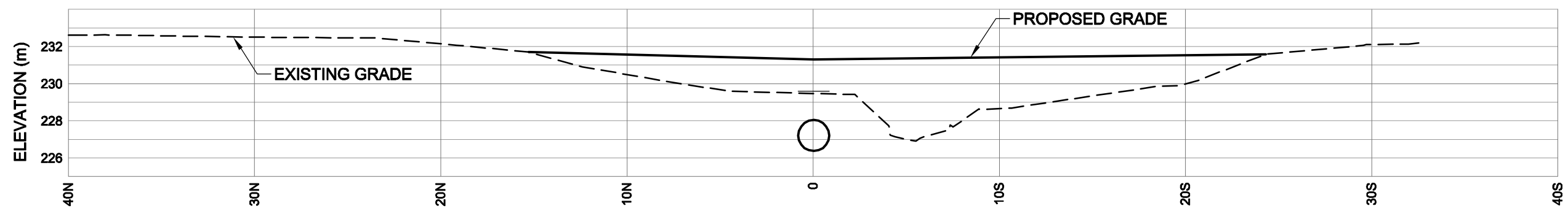
SECTION 1+001 0 2.5 5 7.5 m SCALE 1:250
