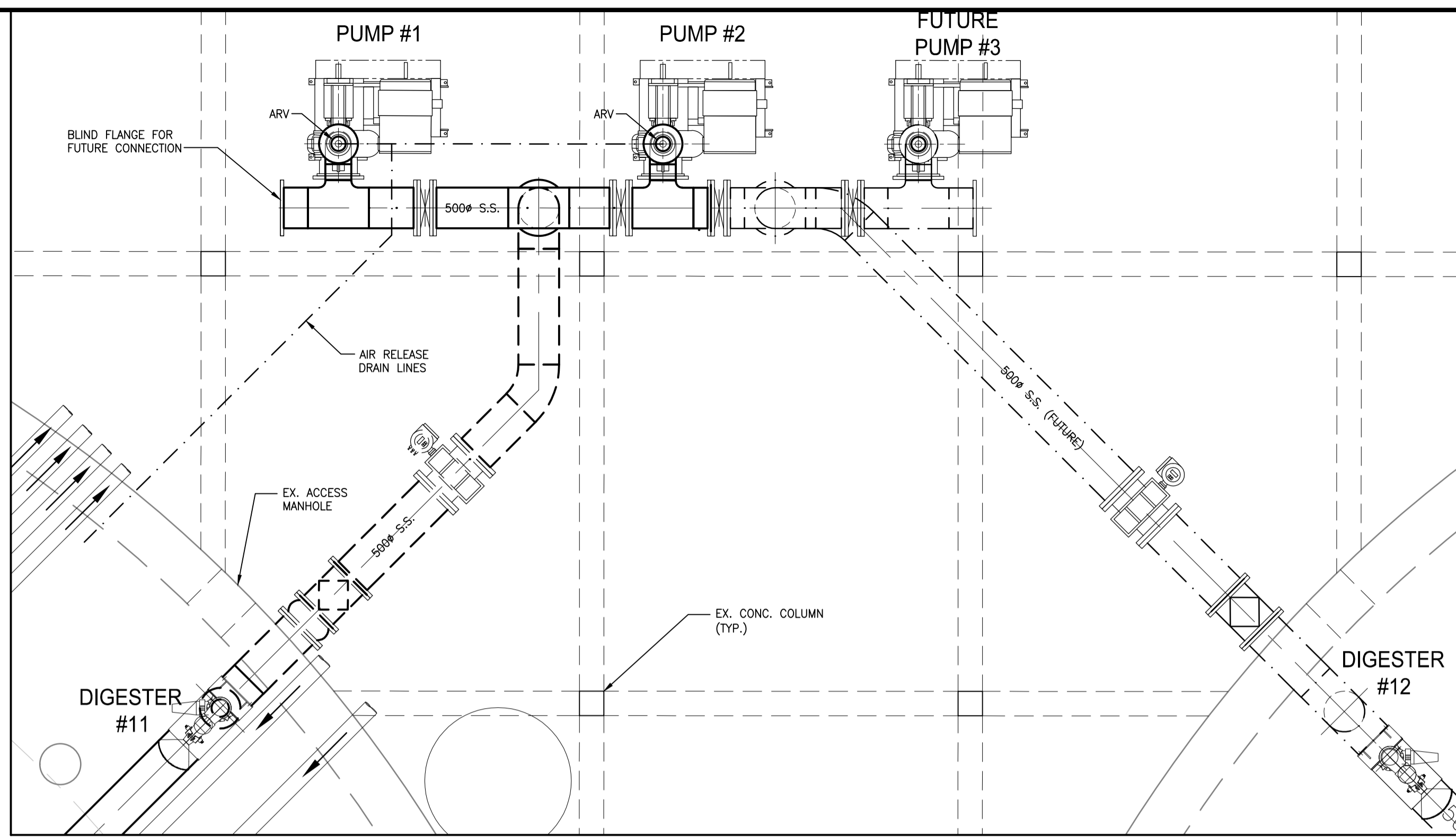
1 SUCTION LINE PLAN 1:50
