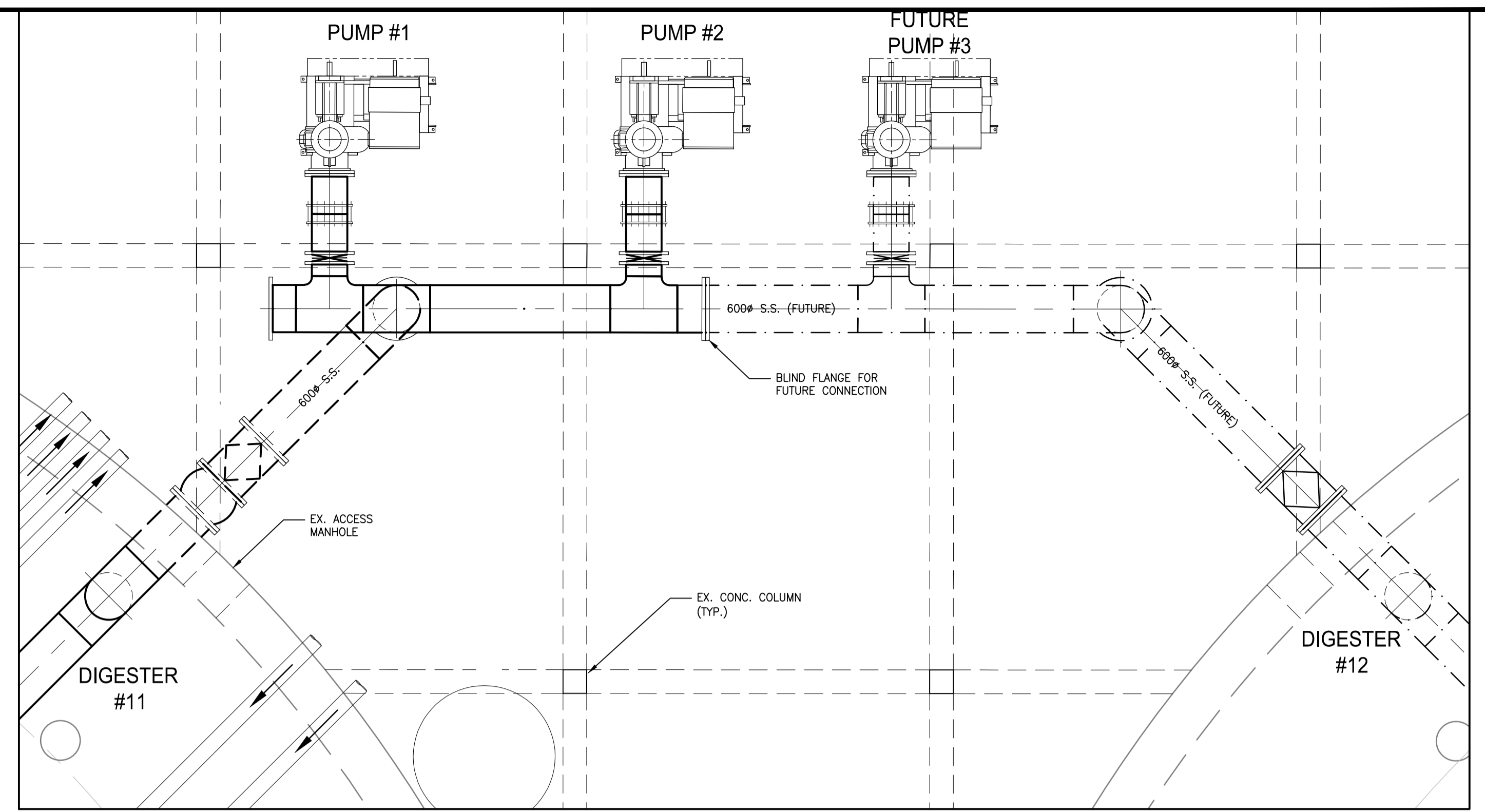
2 DISCHARGE LINE PLAN 1:50
