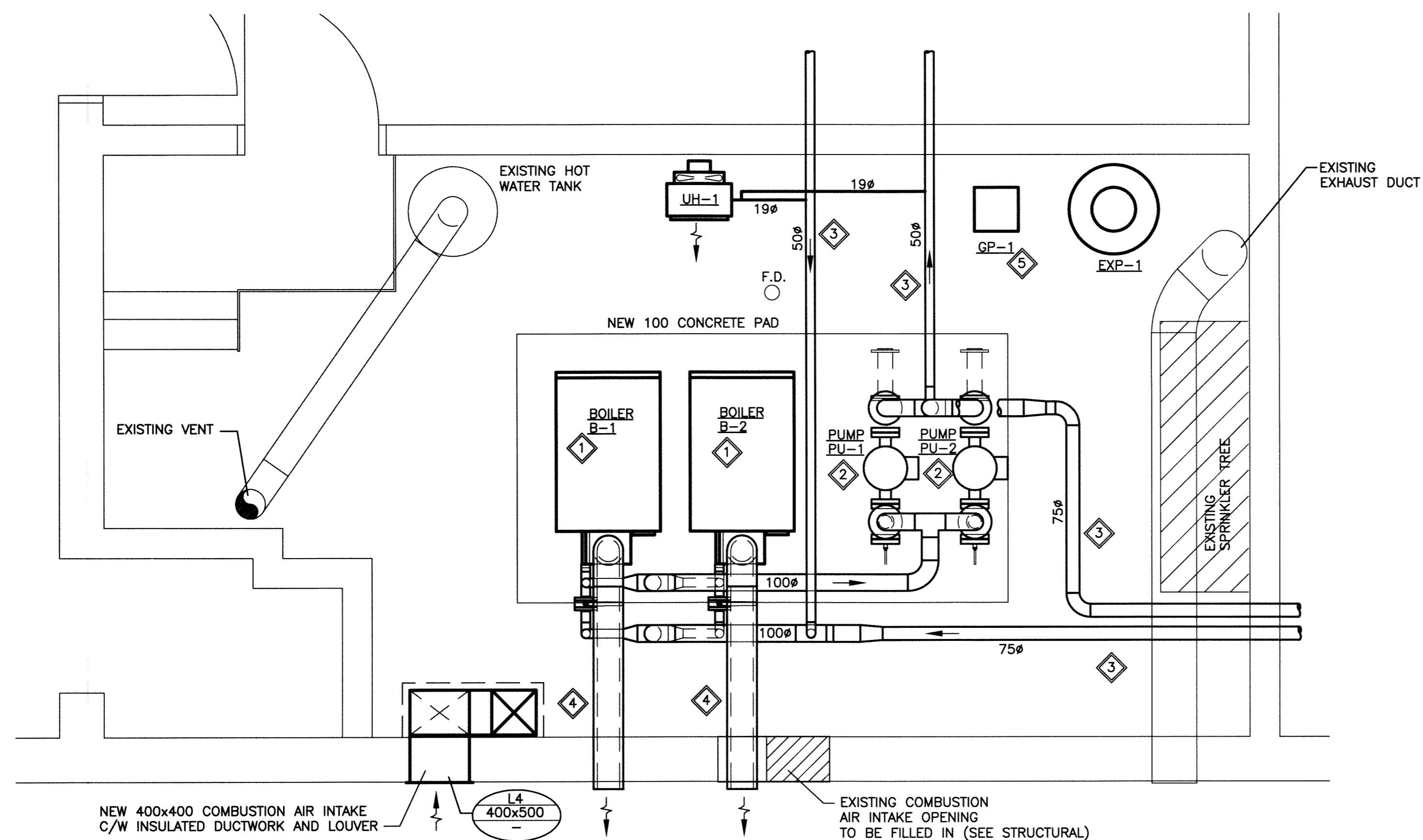
BOILER ROOM PLAN 500 0 500 1000 1500 2000 SCALE: 1:25mm
