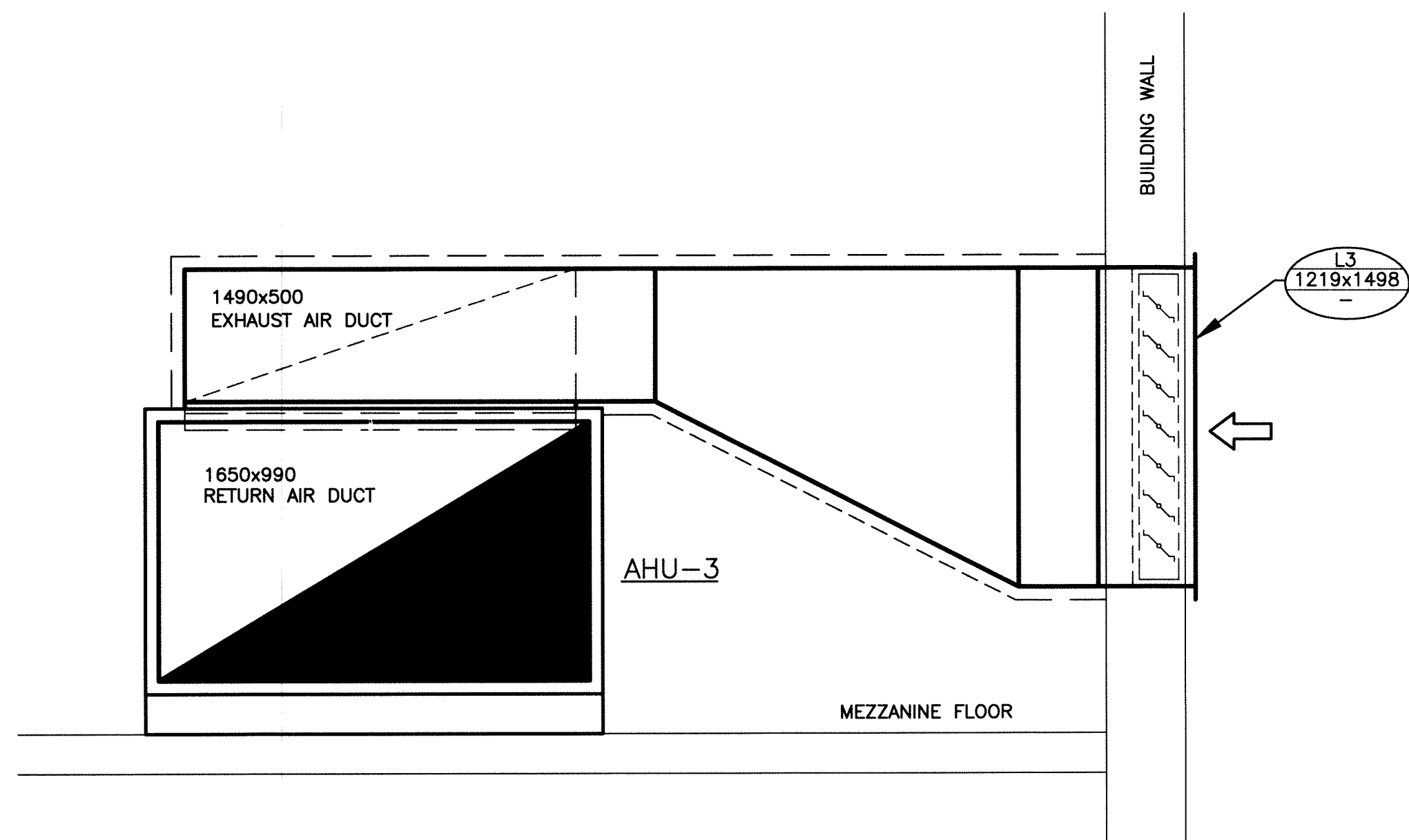
A SECTION - AHU-3 P2-M08 400 0 400 800 1200 1600 SCALE: 1:20mm
