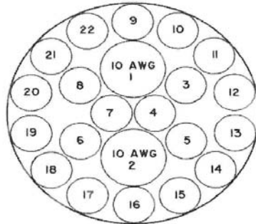
22 - CONDUCTOR CABLE CROSS SECTIONAL VIEW
