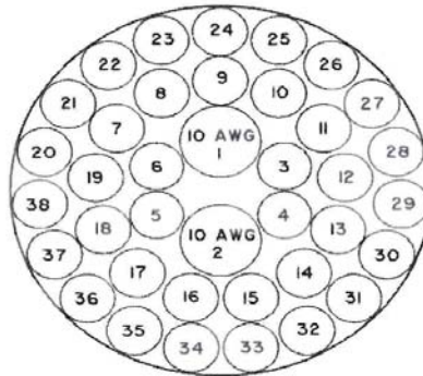
38 - CONDUCTOR CABLE CROSS SECTIONAL VIEW
