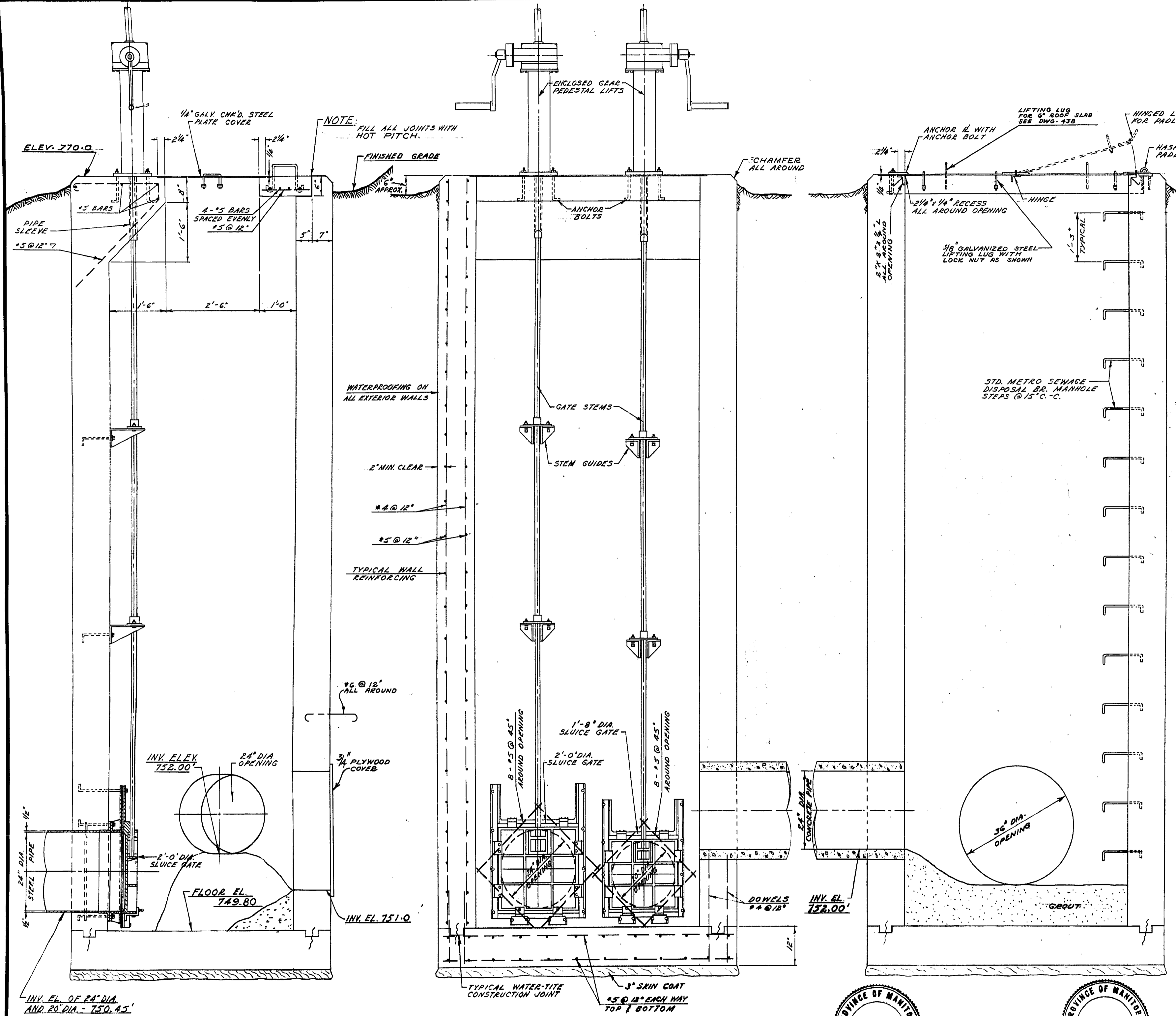
SEC. "A-A"
