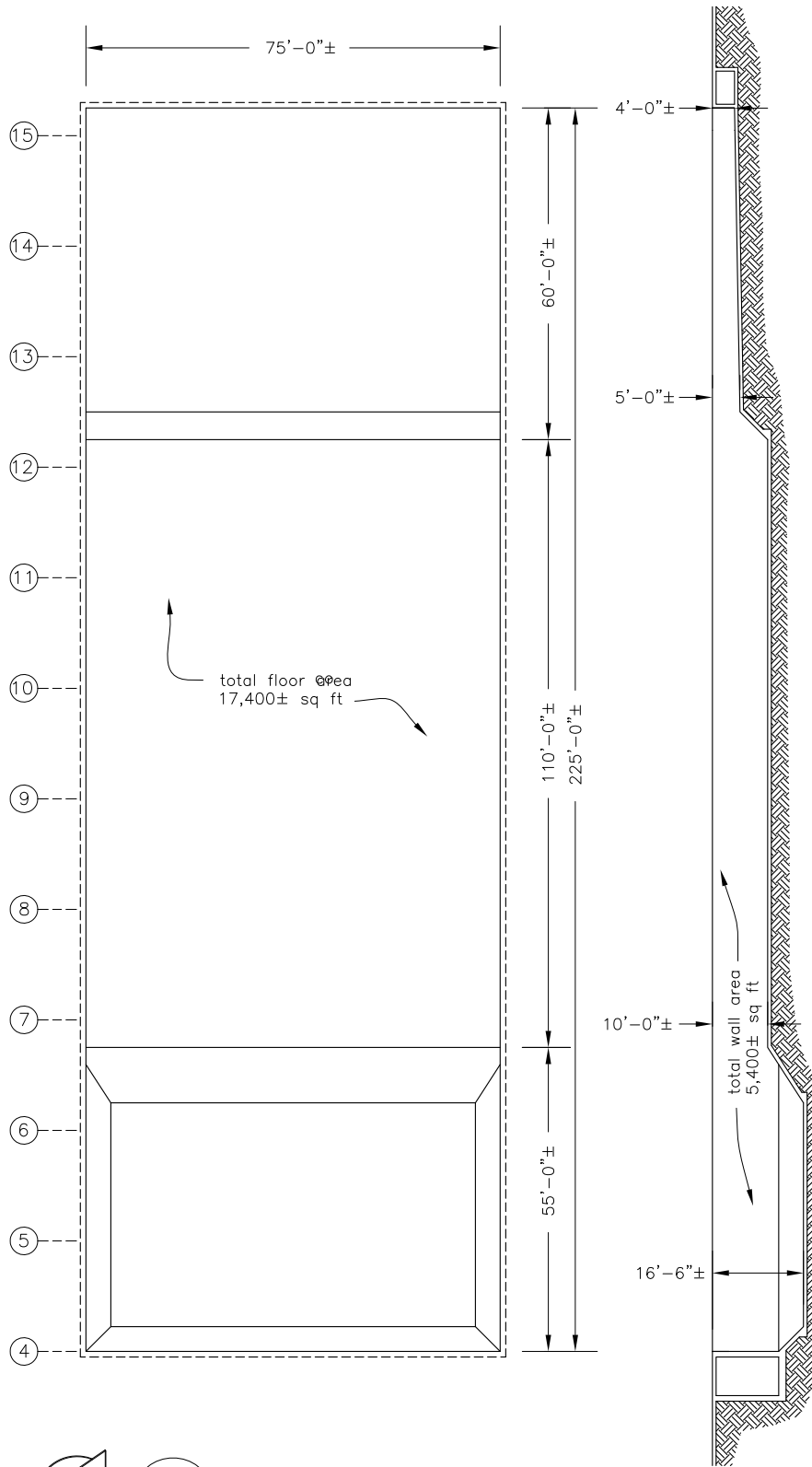
MAIN POOL TANK PLAN SCALE: 1/32" = 1'-0"
