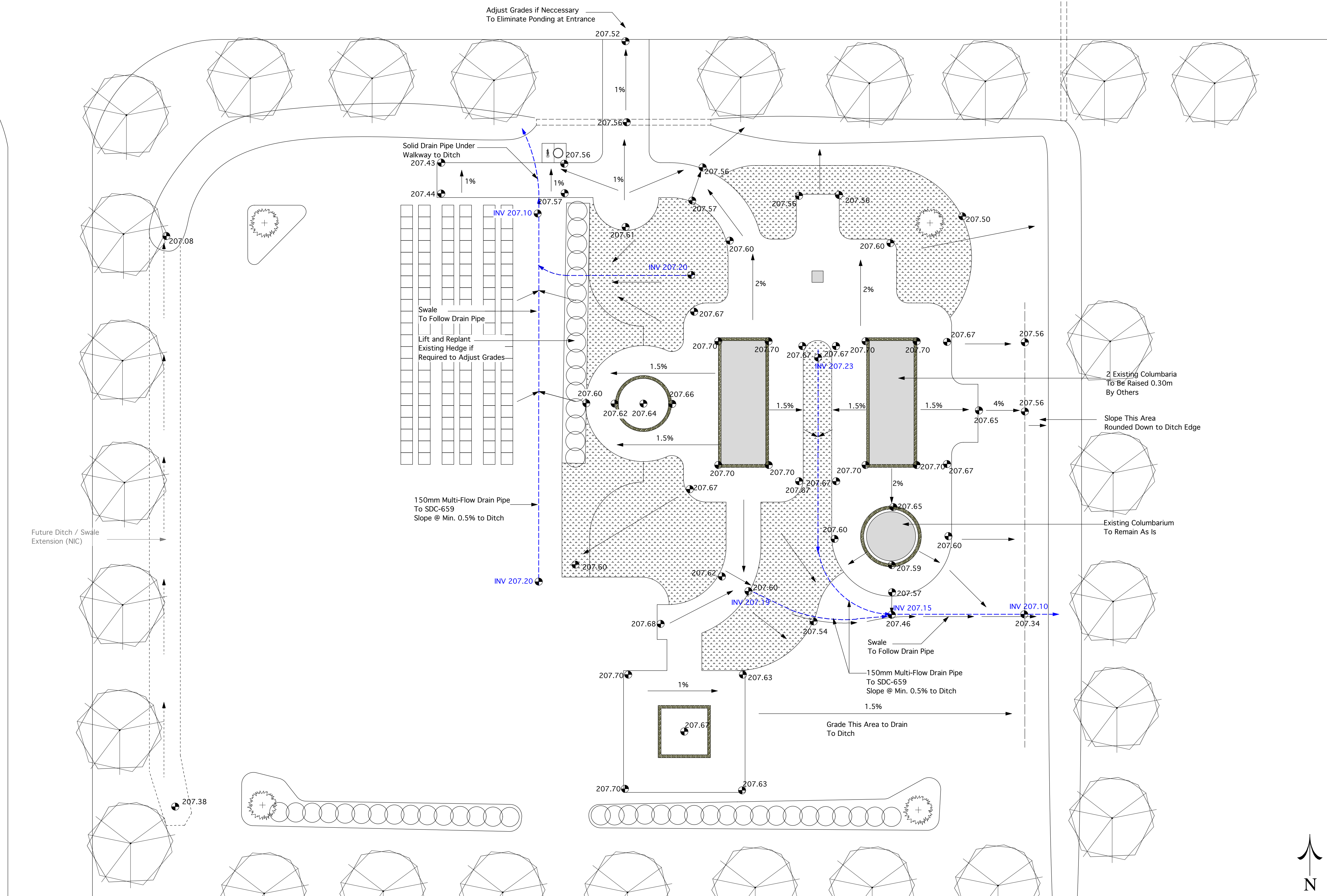
1 GRADING SCHEMATIC PLAN L4 1:100
