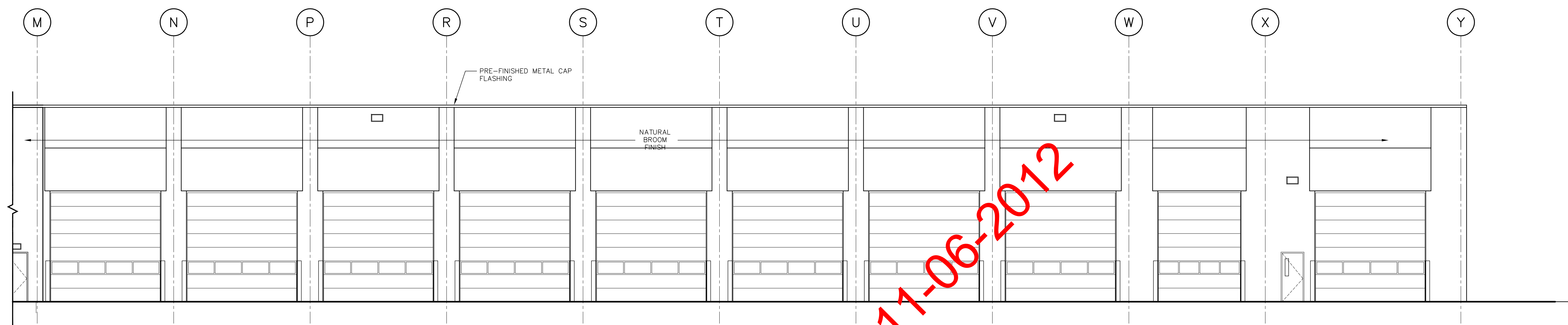
7 WEST BUILDING ELEVATION CONT. 4.4 SCALE 1:100
