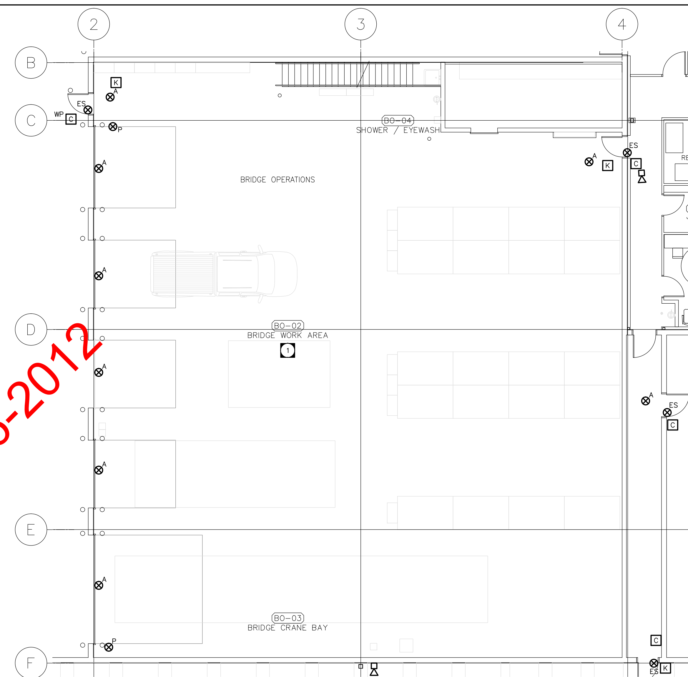
2 E3.1 BRIDGE OPERATIONS FLOOR PLAN - POWER AND SYSTEMS LAYOUT SCALE: 1100
