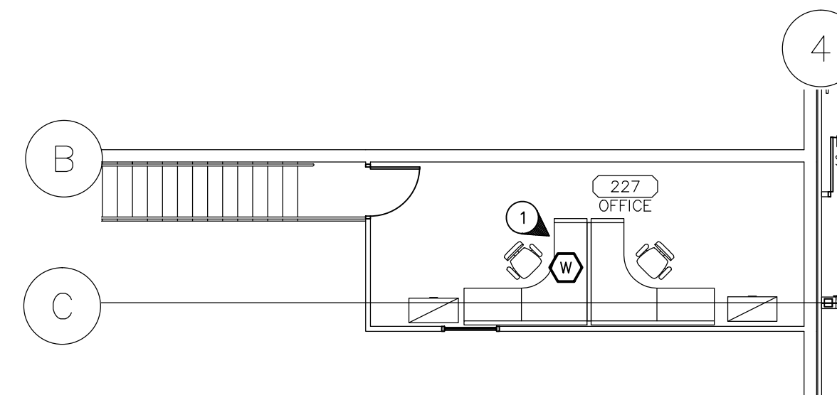
3 E3.12 MEZZANINE FLOOR PLAN BRIDGE OPERATIONS - SECURITY LAYOUT SCALE: 1100
