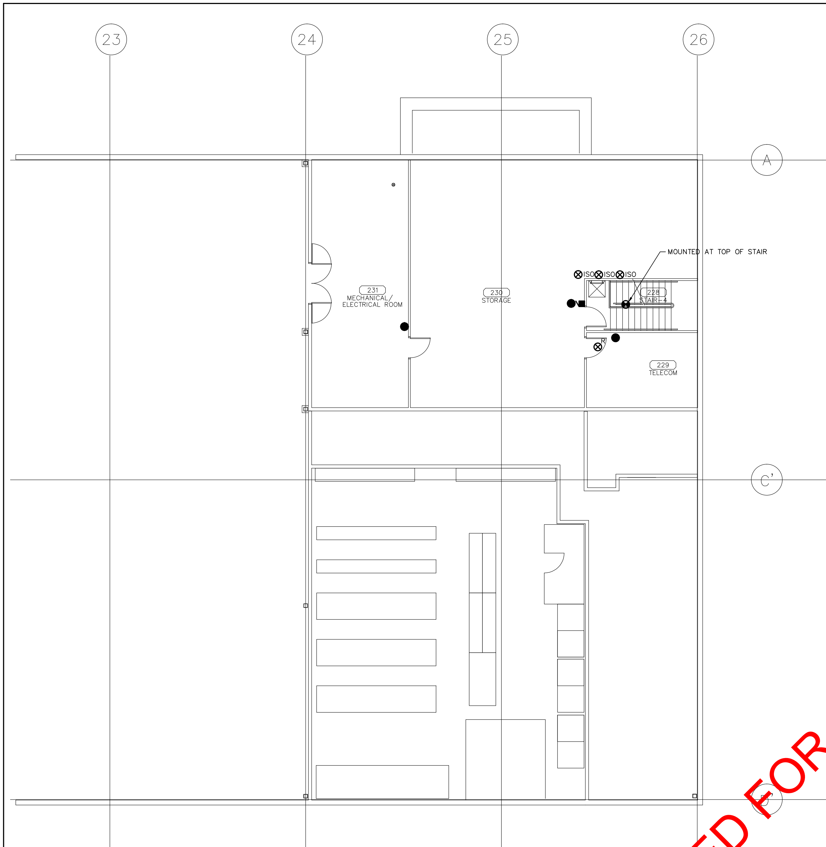
1 E3.5.1 PARTIAL SECOND FLOOR PLAN FLEET MANAGEMENT - FIRE LAYOUT SCALE: 1/100
