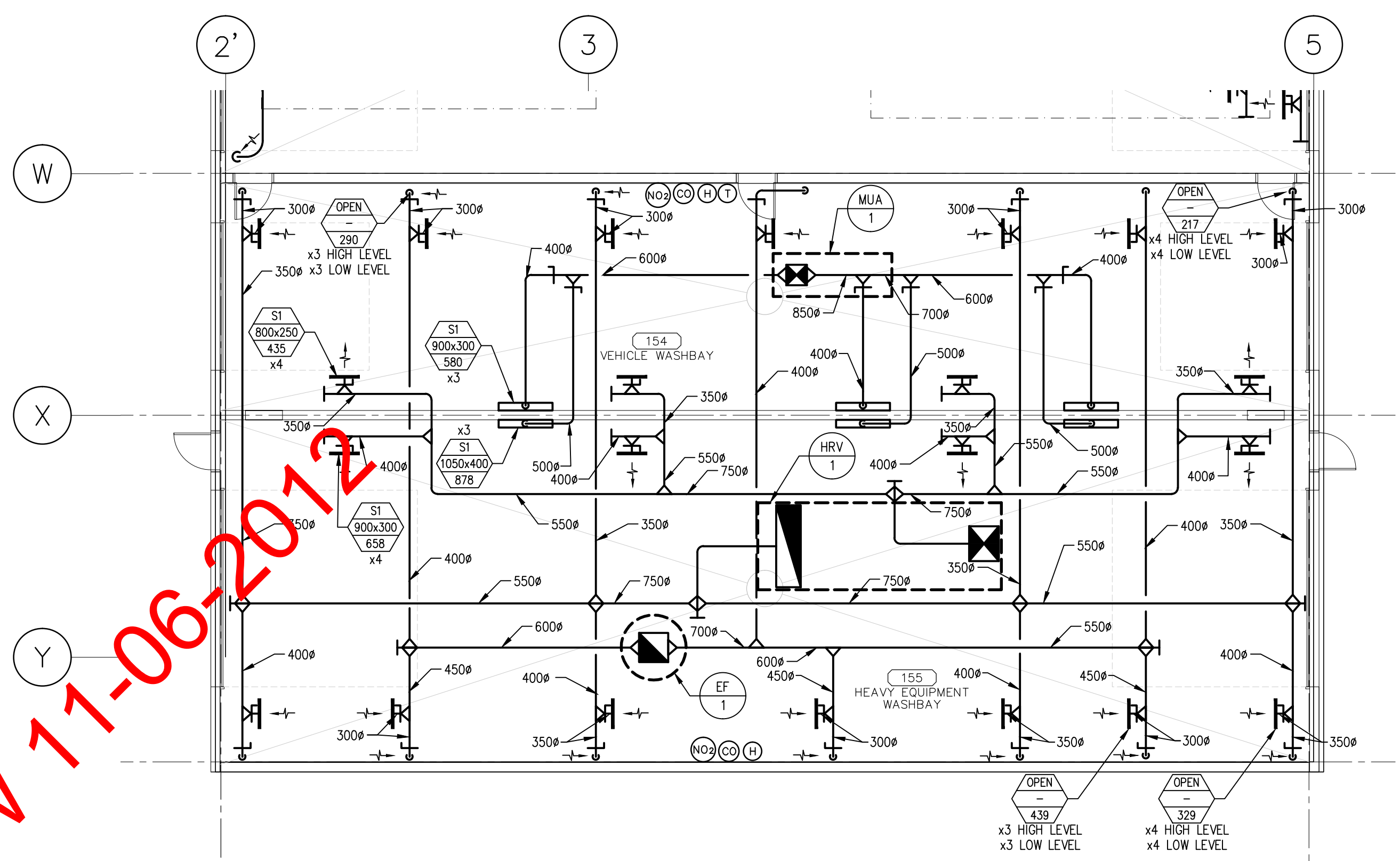
MAIN FLOOR PLAN - H.V.A.C. SCALE 1:100
