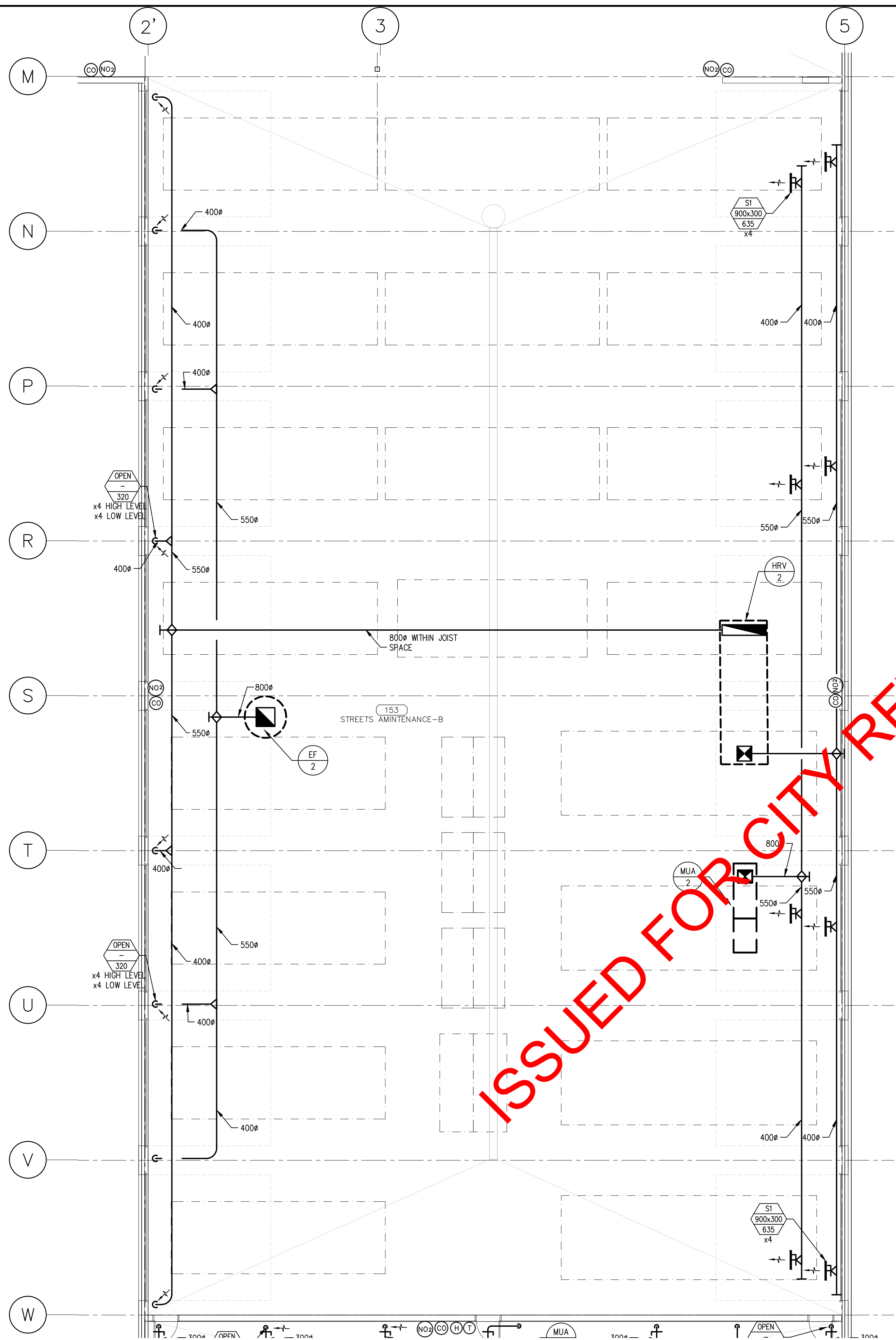
MAIN FLOOR PLAN - H.V.A.C. SCALE 1:100
