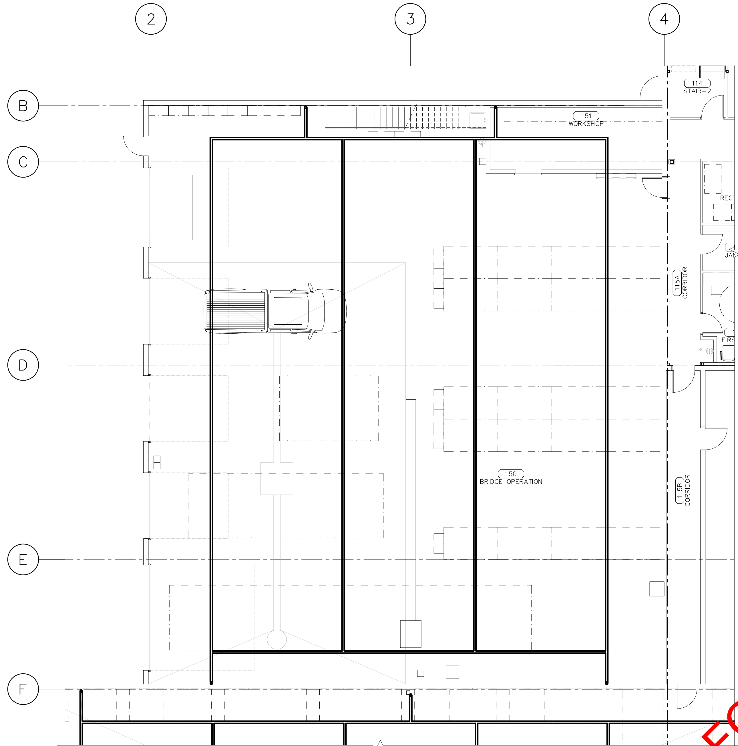
MAIN FLOOR PLAN - METHANE EXTRACTION SCALE 1:100 NOTE: REFER TO INSTALLATION DETAILS ON MECHANICAL DRAWING M4.1
