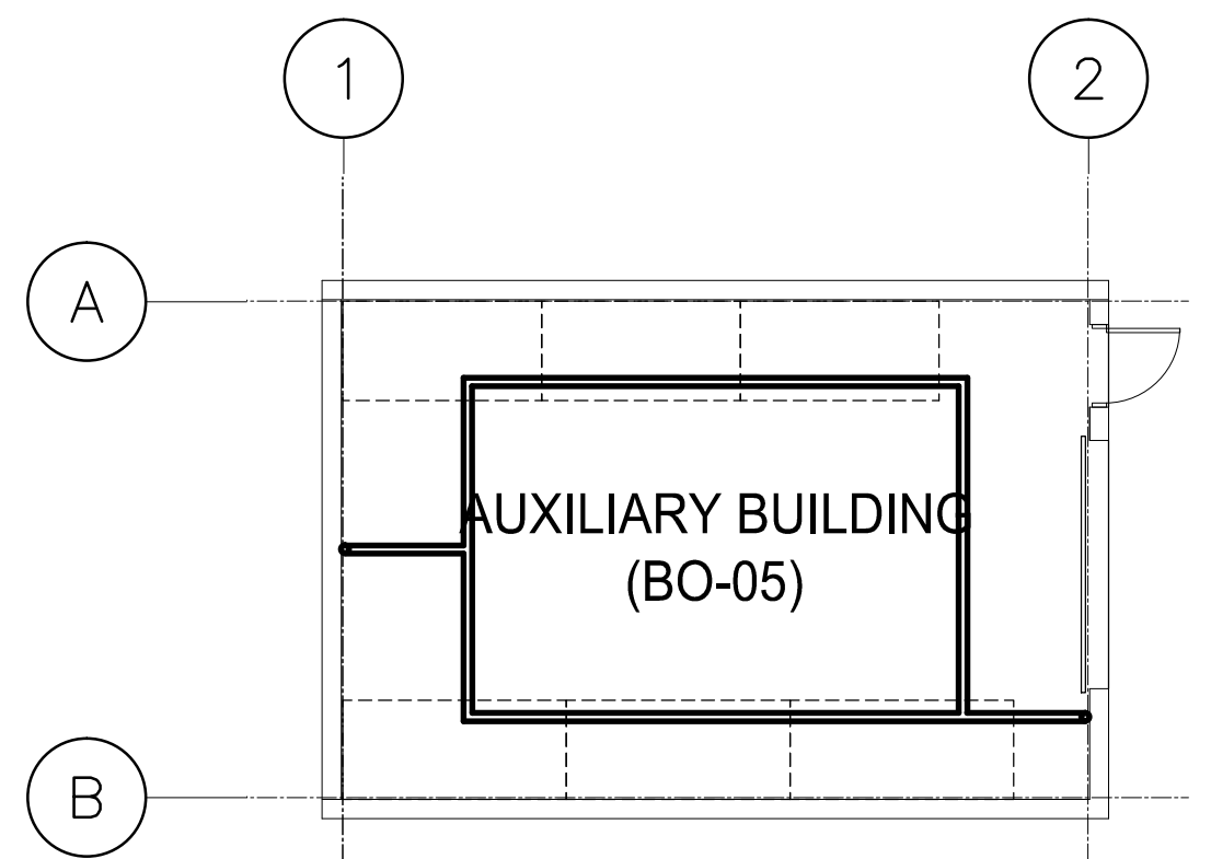
MAIN FLOOR PLAN - METHANE EXTRACTION SCALE 1:100
