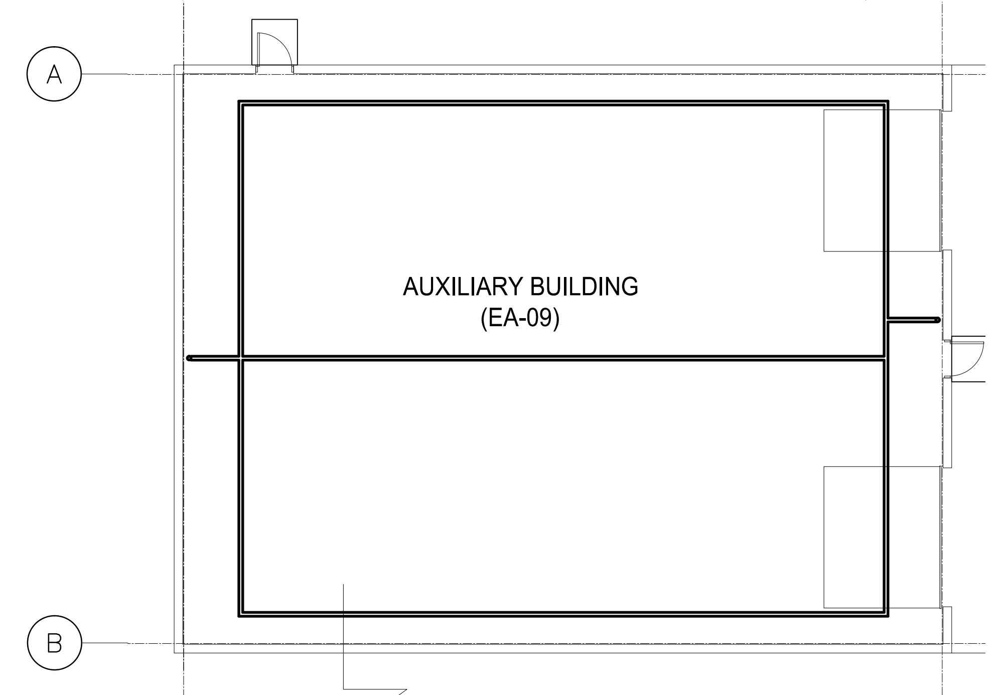
MAIN FLOOR PLAN - METHANE EXTRACTION SCALE 1:100
