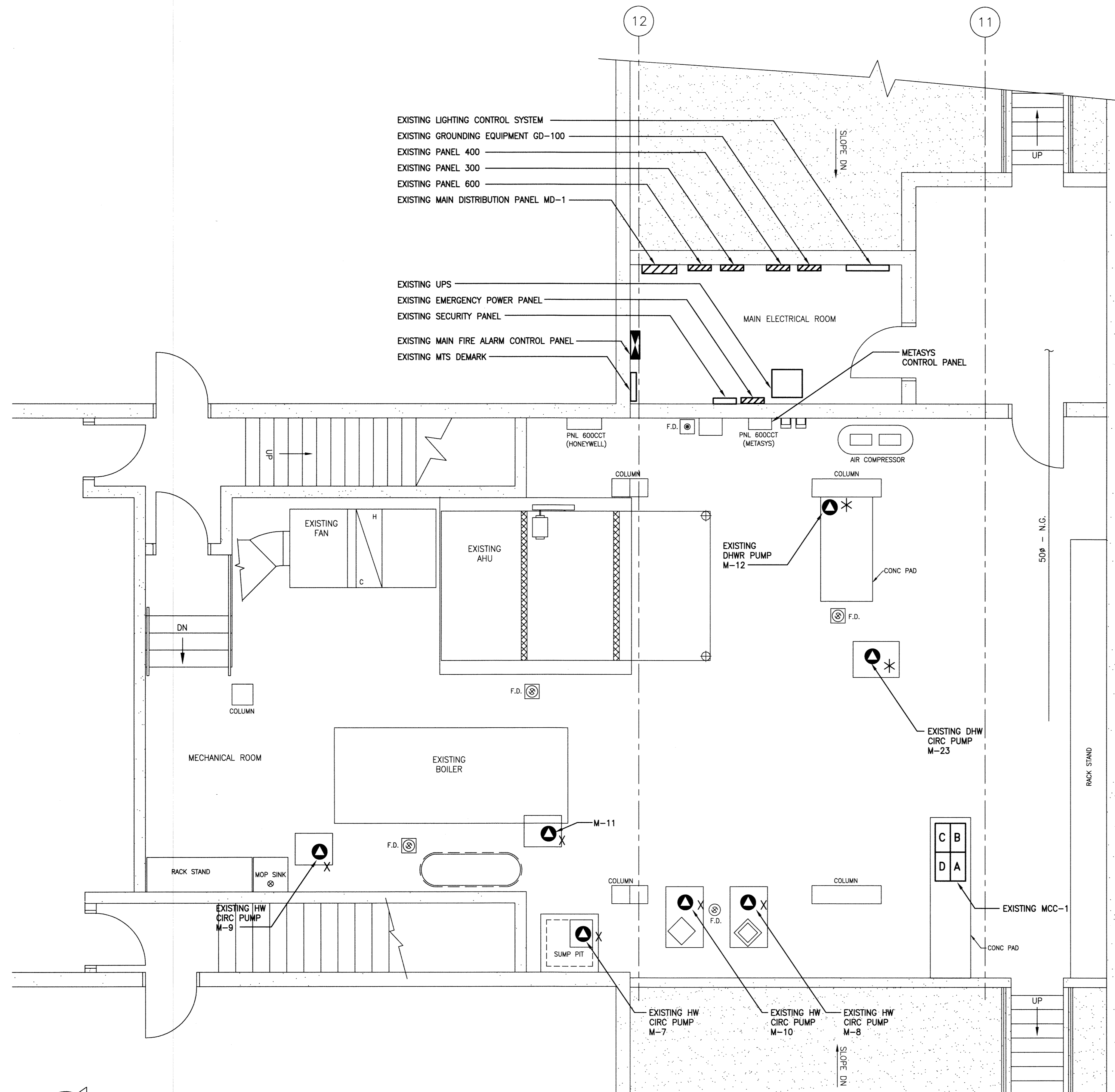
1 BASEMENT MECHANICAL ROOM PLAN - DEMOLITION 800 0 800 1600 2400 3200 SCALE: 1:40mm
