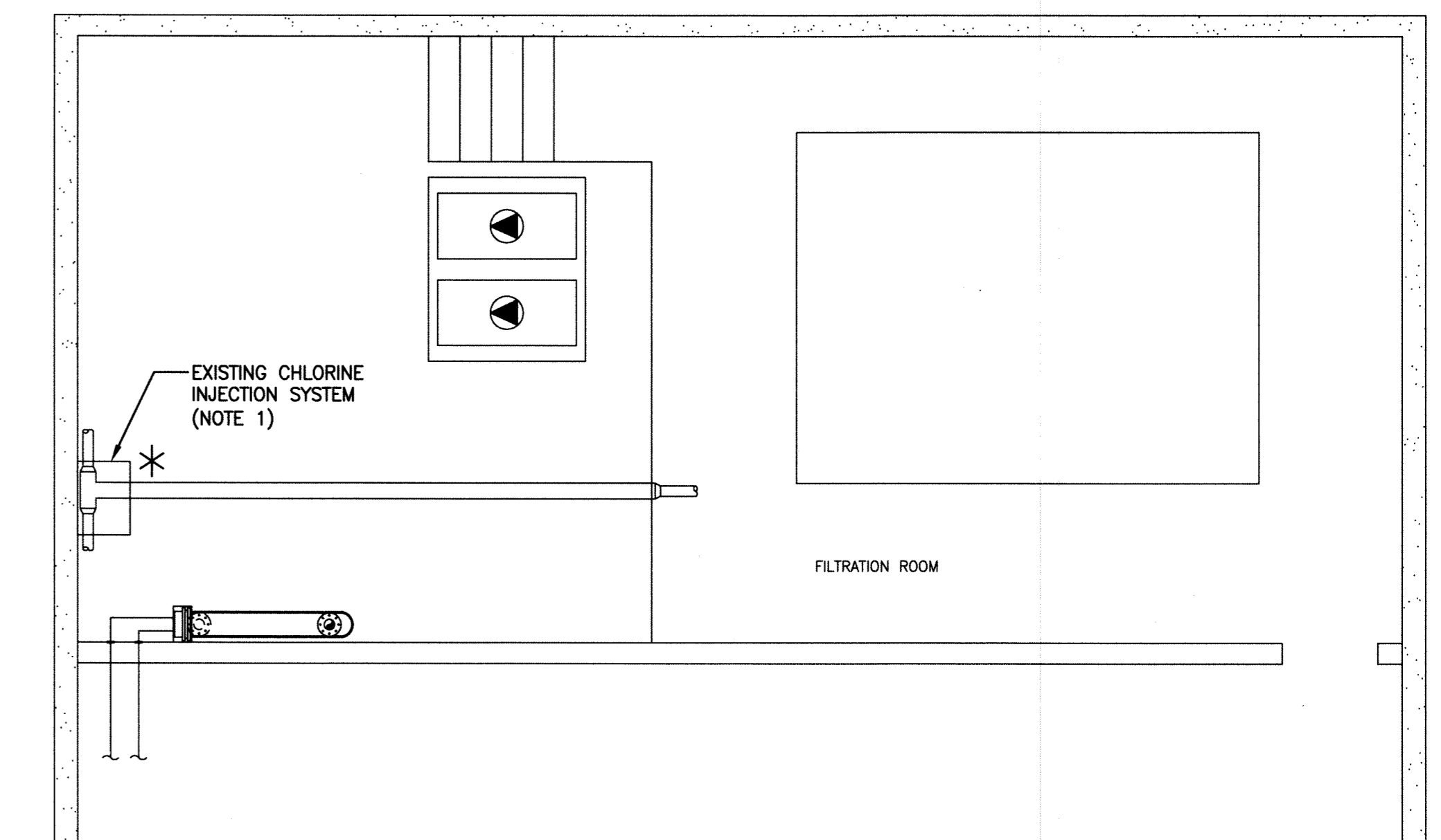
2 BASEMENT FILTRATION ROOM PLAN - DEMOLITION 1000 0 1000 2000 3000 4000 SCALE: 1:50mm
