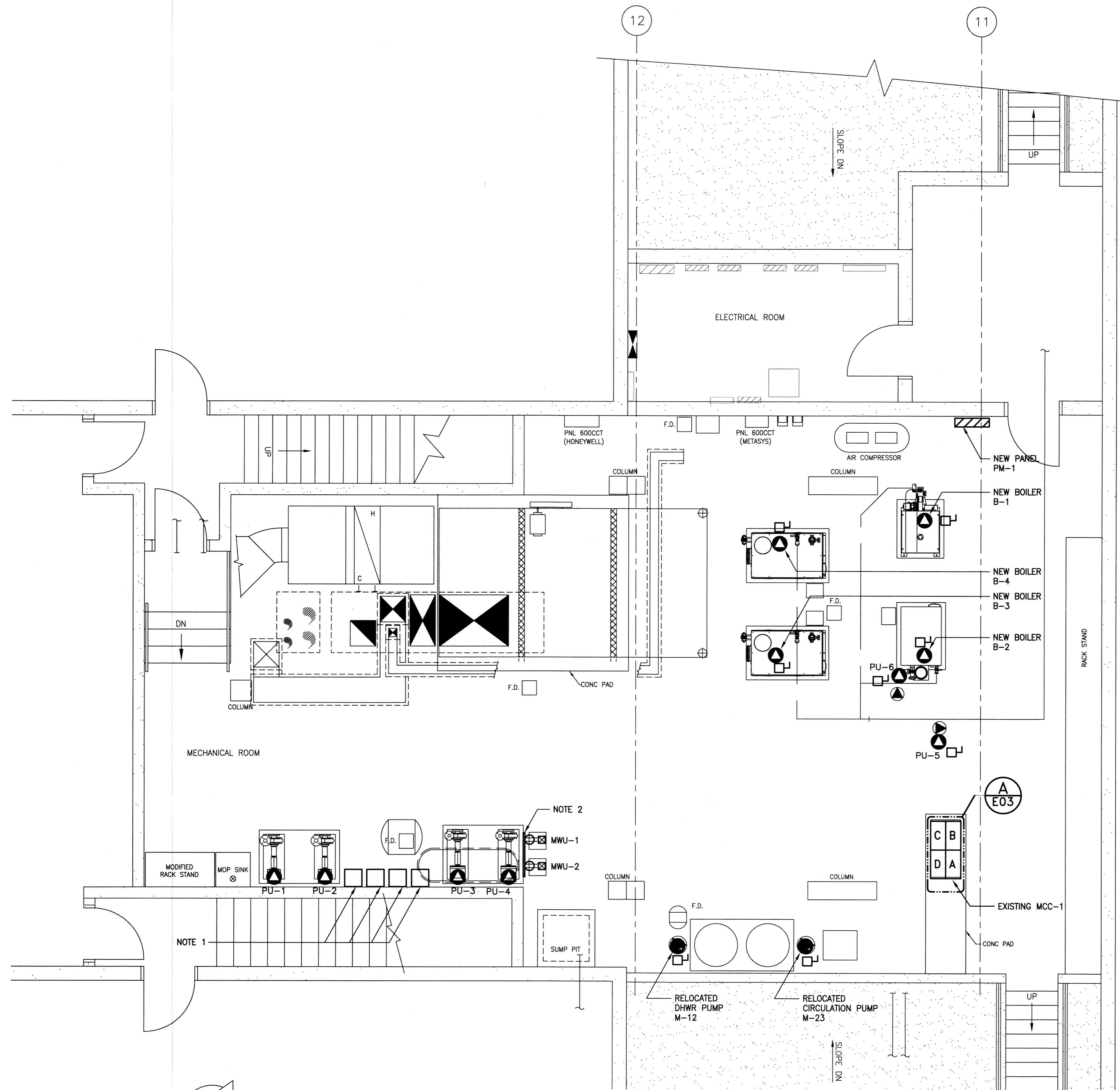
1 BASEMENT MECHANICAL ROOM PLAN - NEW 800 0 800 1600 2400 3200 SCALE: 1:40mm
