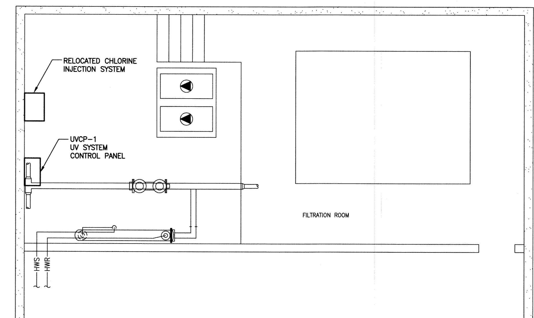
2 BASEMENT FILTRATION ROOM PLAN - NEW 1000 0 1000 2000 3000 4000 SCALE: 1:50mm
