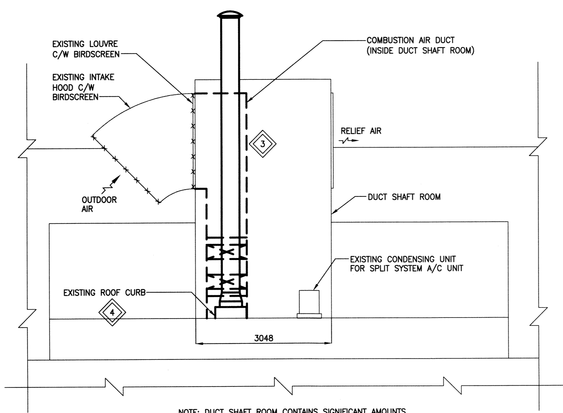
SECTION A-A - NORTH FACE OF BLDG. SCALE: 1:50mm
