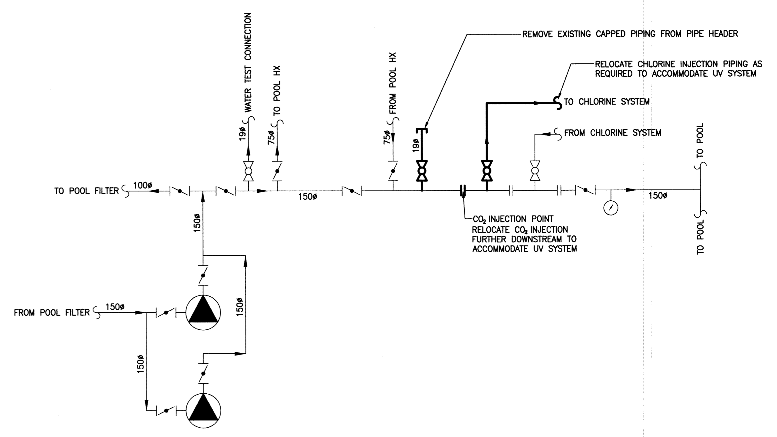
2 POOL WATER PIPING SCHEMATIC - DEMOLITION AND RELOCATION SCALE: N.T.S.
