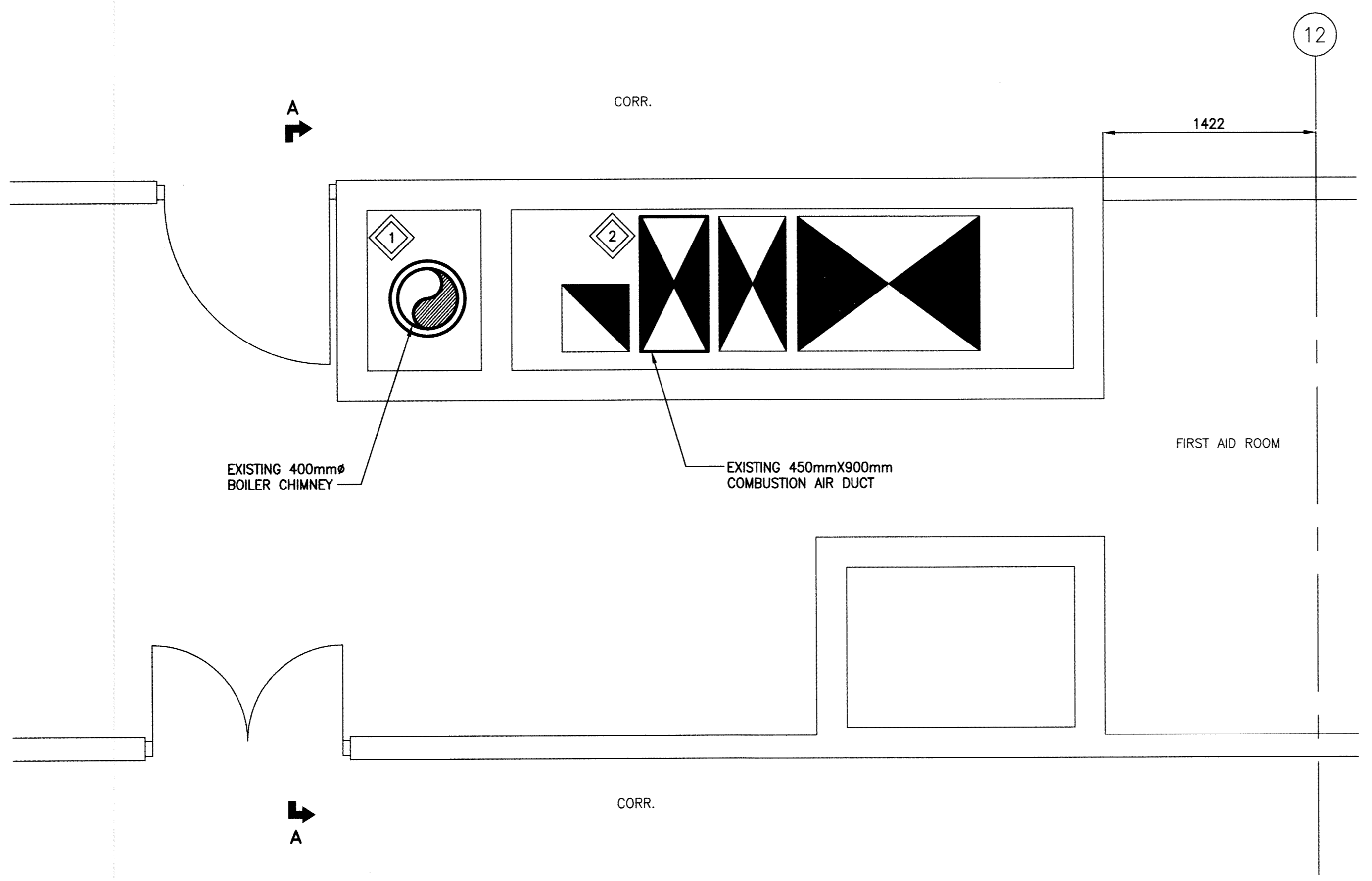
1 PARTIAL MAIN FLOOR PLAN - HVAC DEMOLITION SCALE: 1:25mm
