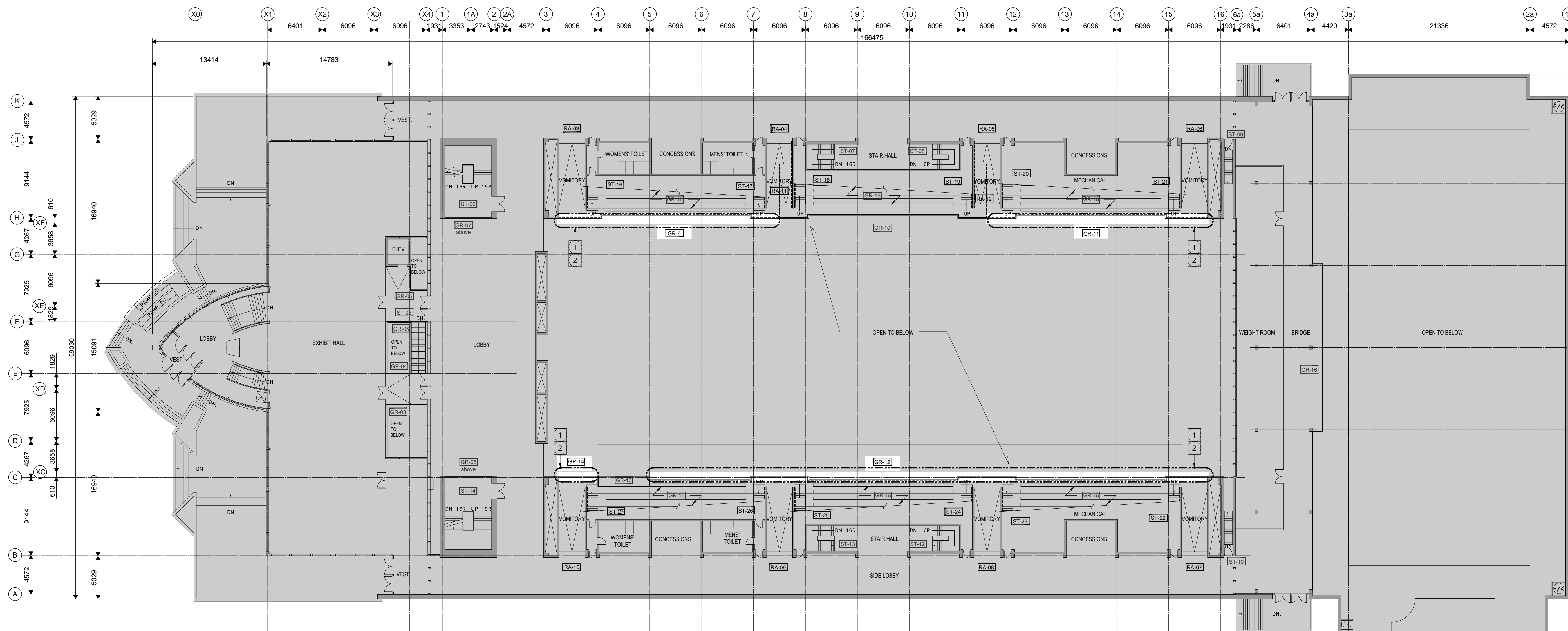
2 SECOND FLOOR KEY PLAN A-2.1 Scale 1:500
