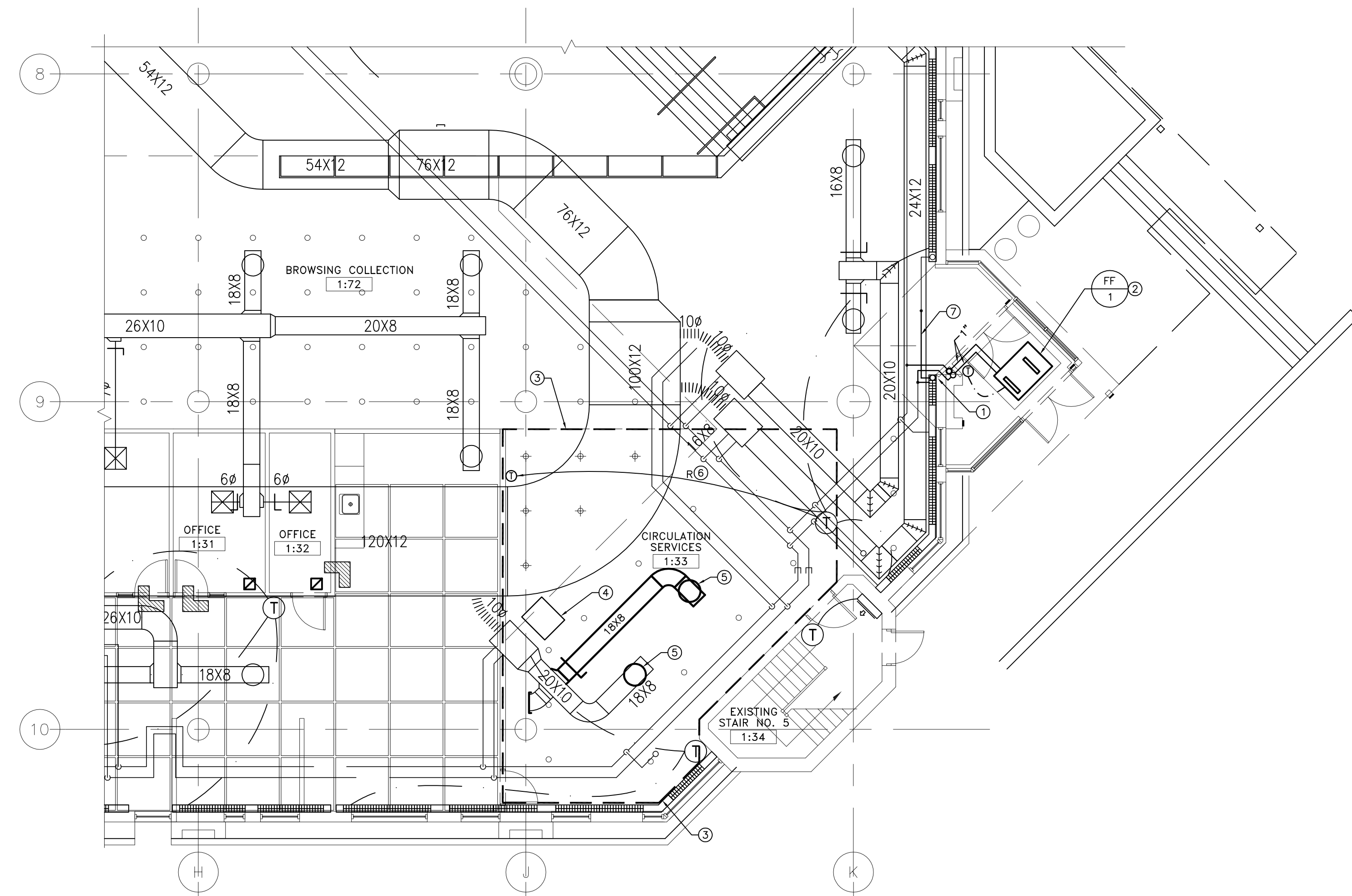
2 RENOVATION PLAN - HVAC M2.0 SCALE: 1/8"=1'-0"
