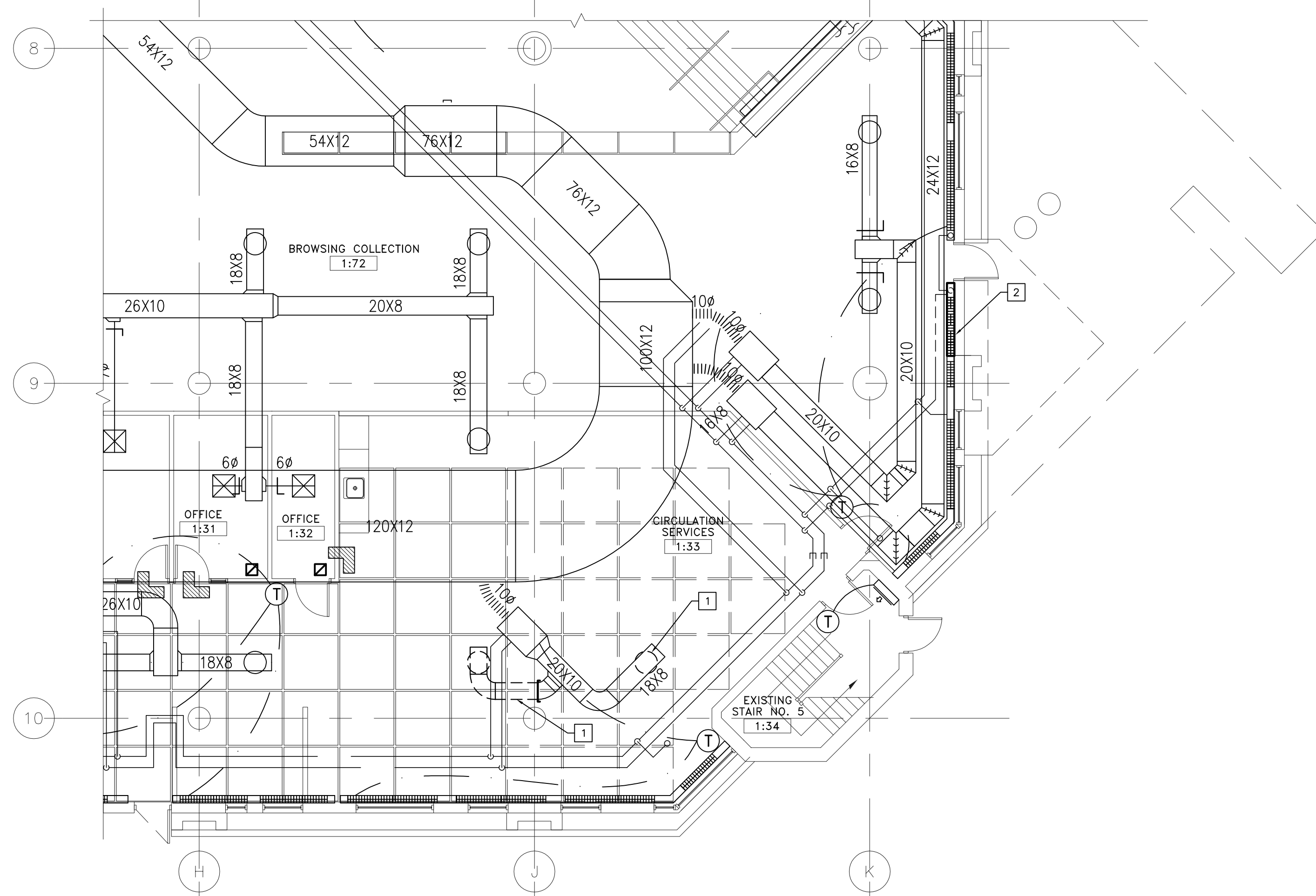
1 DEMOLITION PLAN - HVAC M2.0 SCALE: 1/8"=1'-0"
