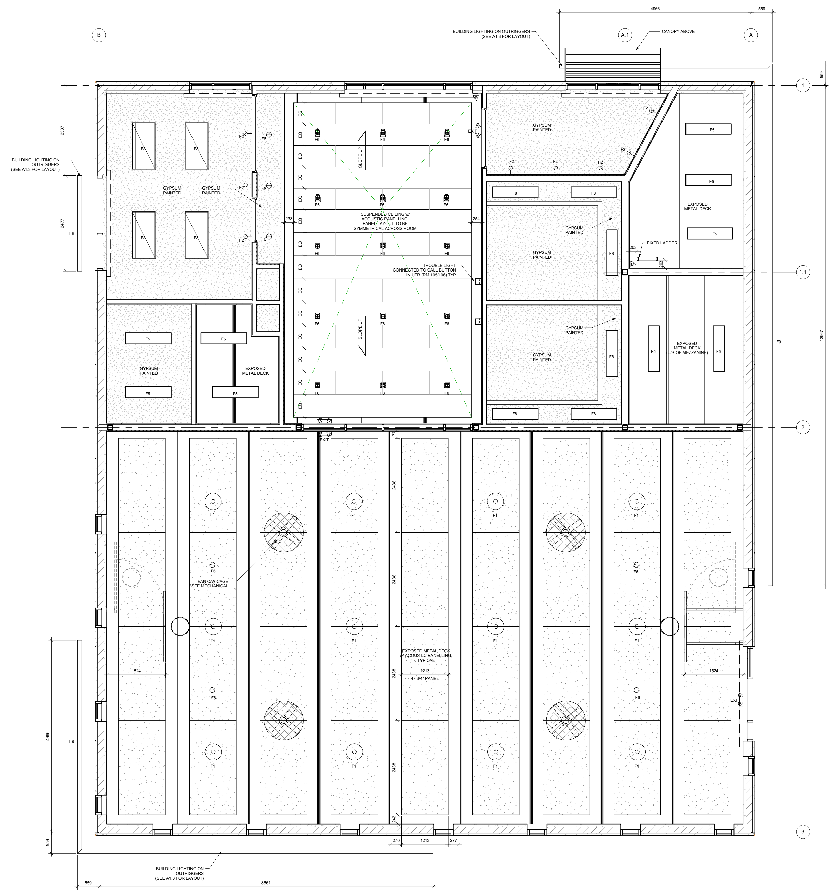
1 MAIN FLOOR RCP A1.2 1:50
