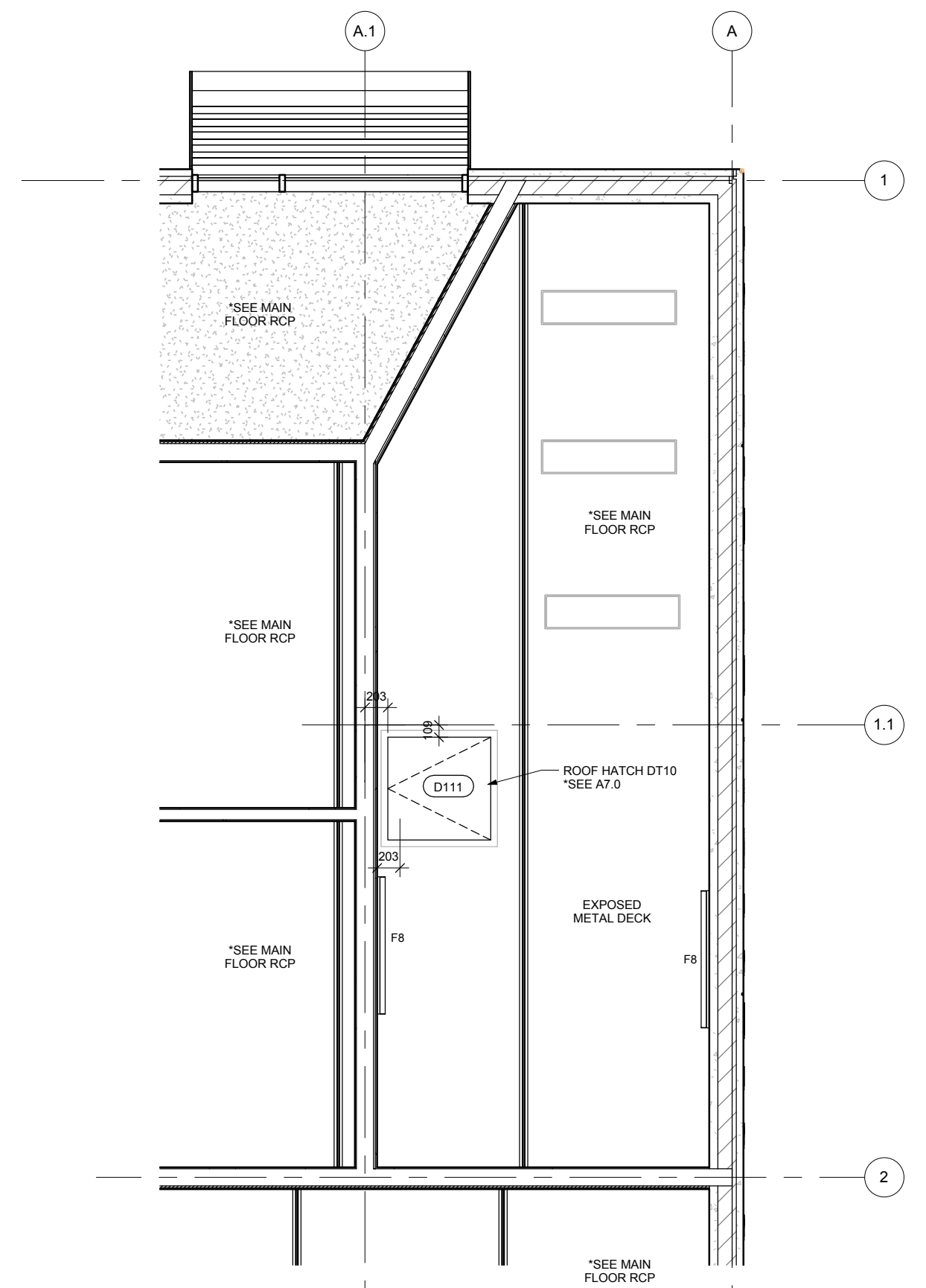
2 ELEVATED MAINTENANCE CATWALK RCP 1:50
