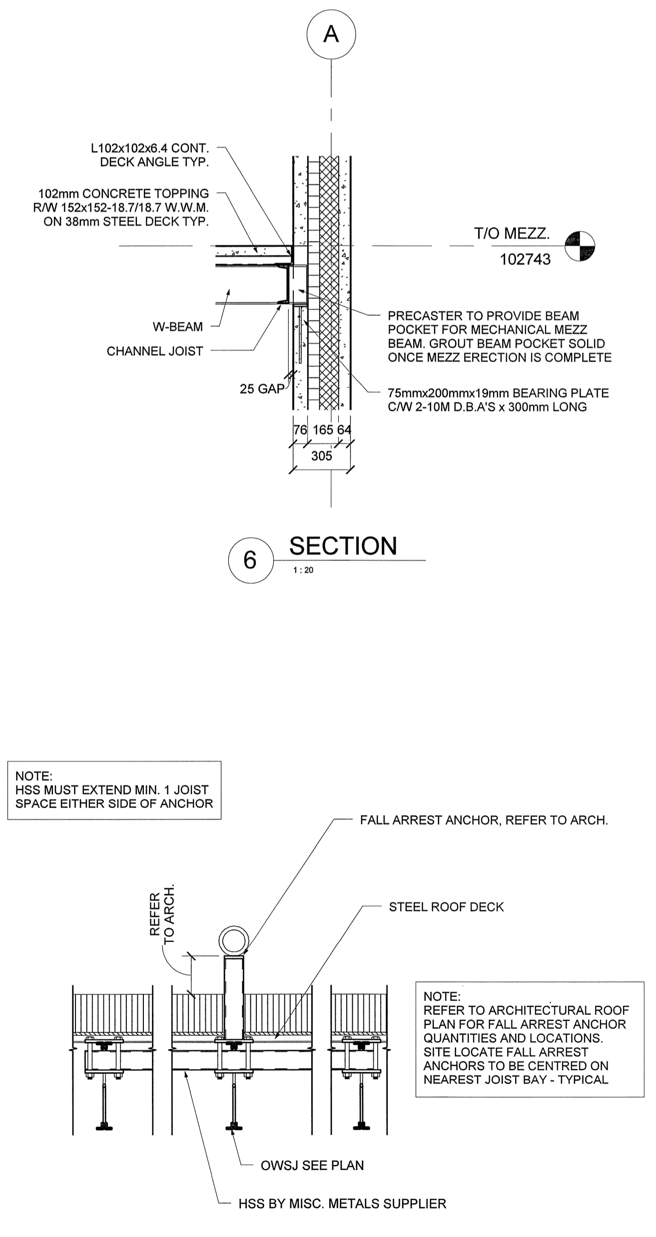
7 TYPICAL ROOF ANCHOR 1:20
