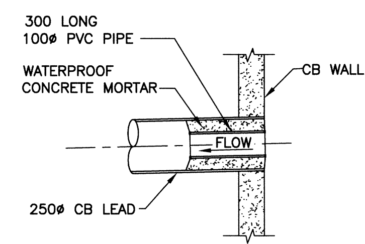
RESTRICTION PIPE DETAIL SCALE: NTS
