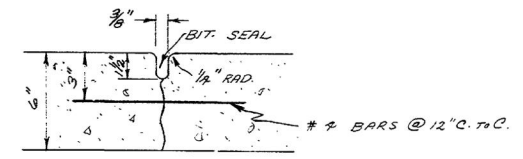
TRANSVERSE CONTRACTION JOINT
