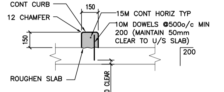
D TYP CONC HOUSEKEEPING PAD & CONC CURB DETAILS 1:20
