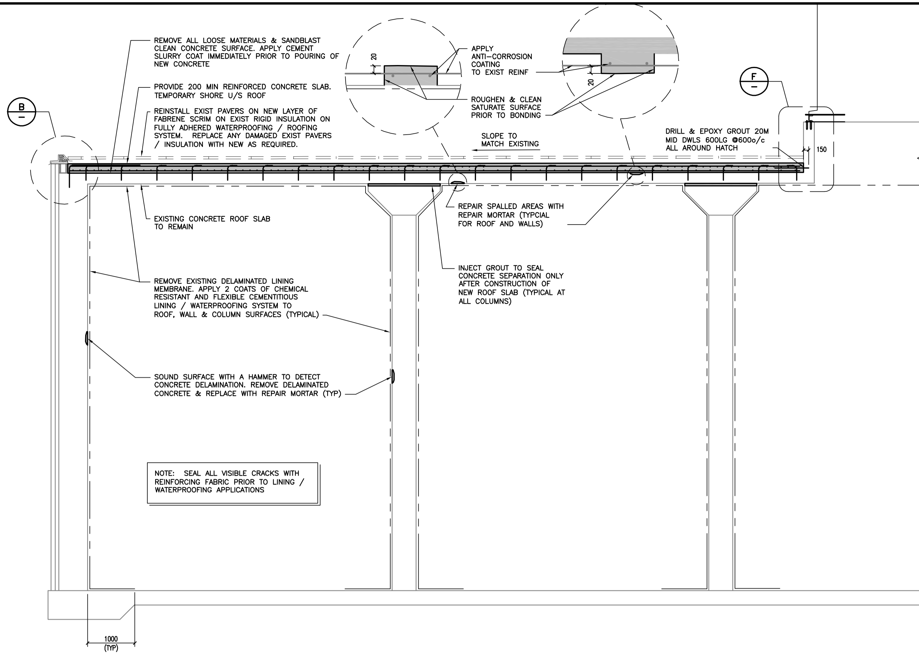
A DIGESTER TANK NO. 11 SECTION 1:50
