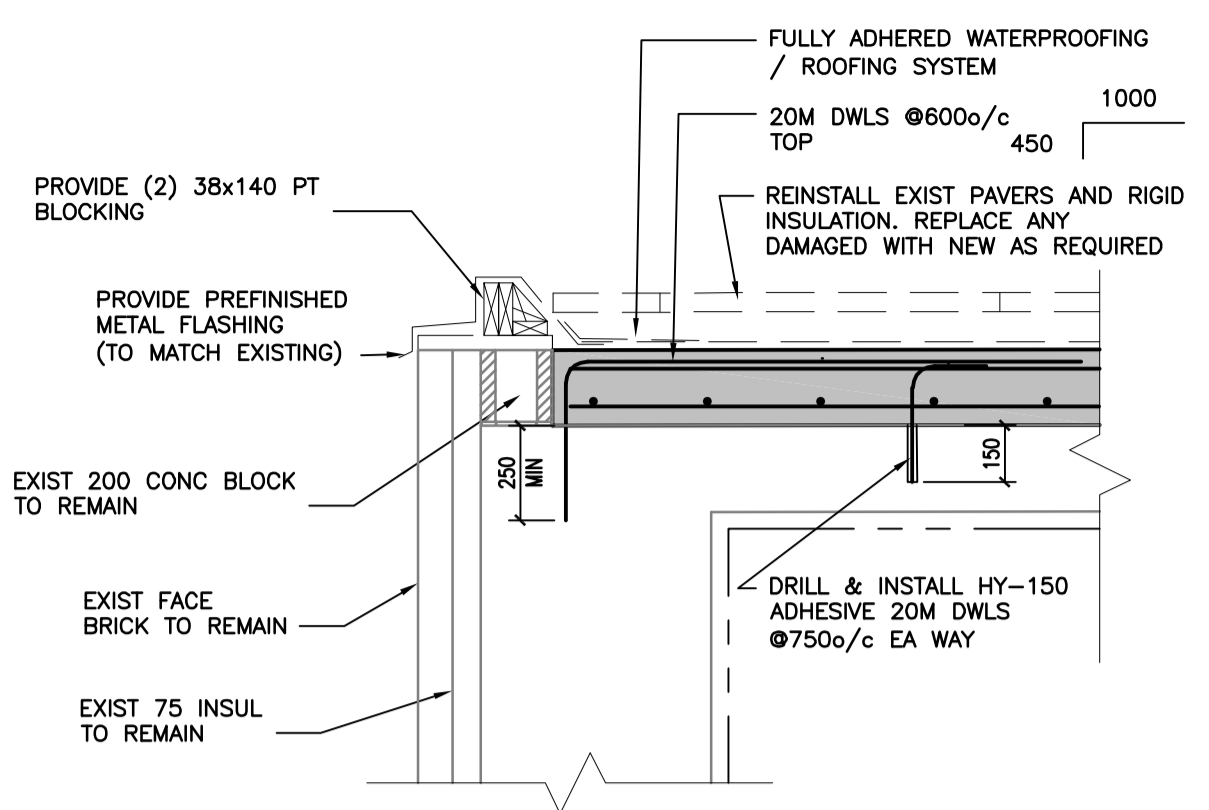
B SECTION 1:20
