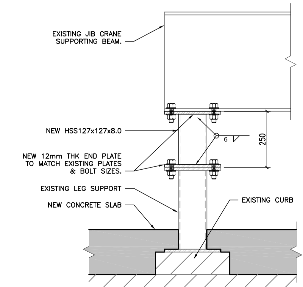
G JIB CRANE CONN SECTION 1:10
