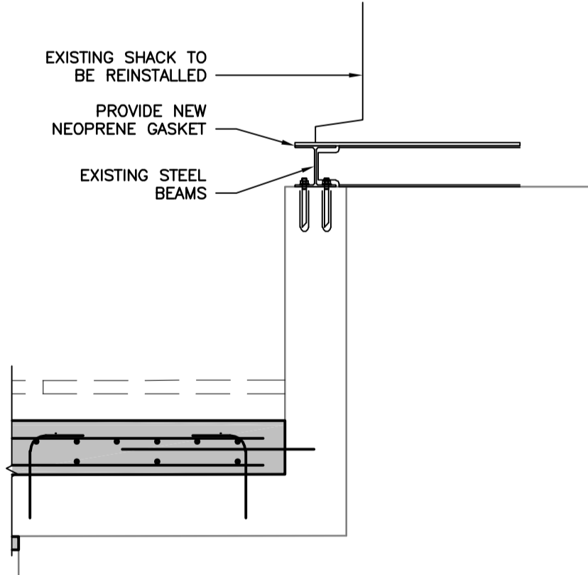
F SECTION 1:20
