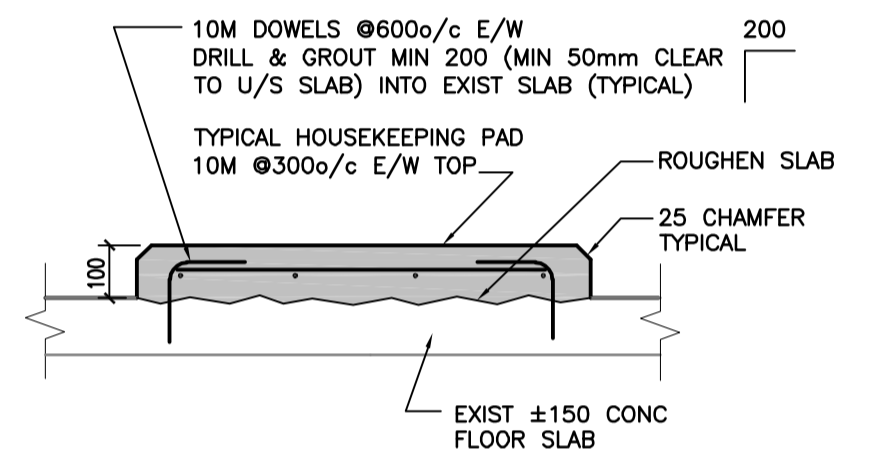
D TYP CONC HOUSEKEEPING PAD & CONC CURB DETAILS 1:20
