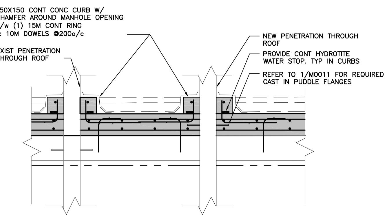
C TYPICAL SAMPLING PORT PENETRATION THROUGH ROOF DETAIL 1:20
