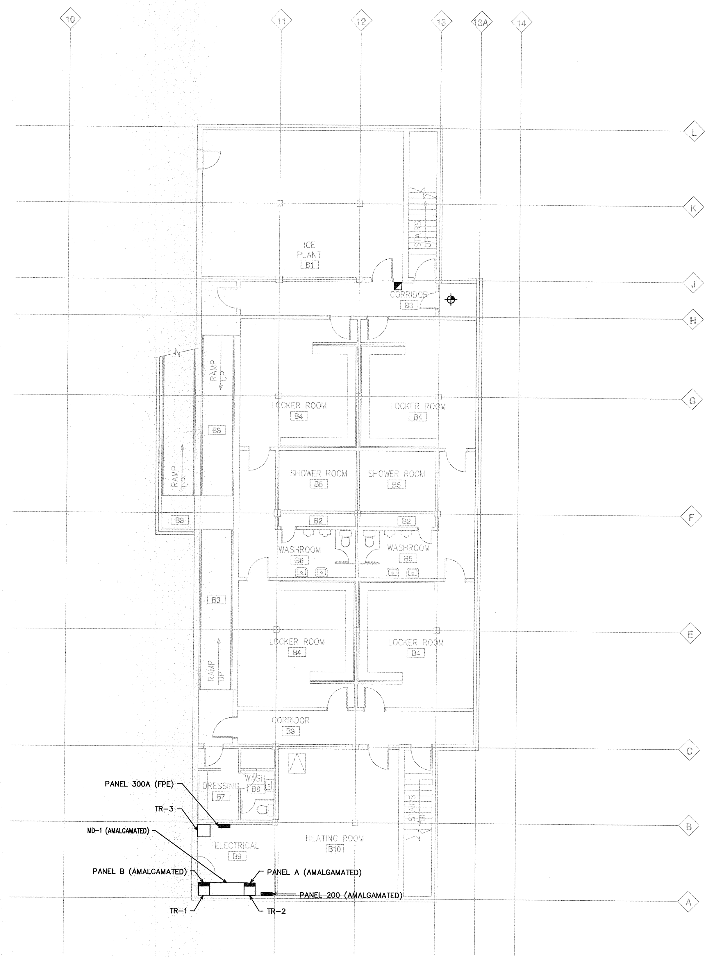
1 BASEMENT POWER & SYSTEMS DEMOLITION LAYOUT EDP2.0 SCALE: 1:100
