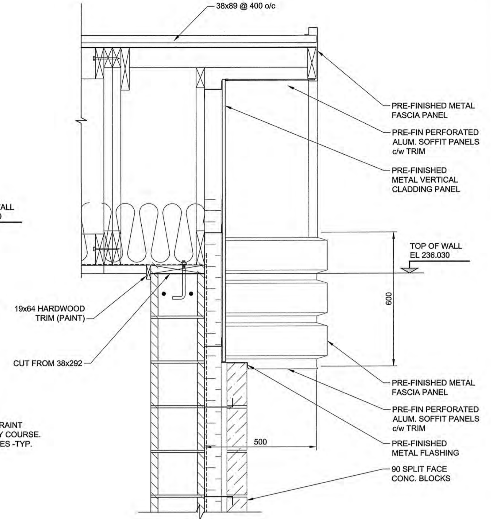
2 DETAIL Scale 1:10
