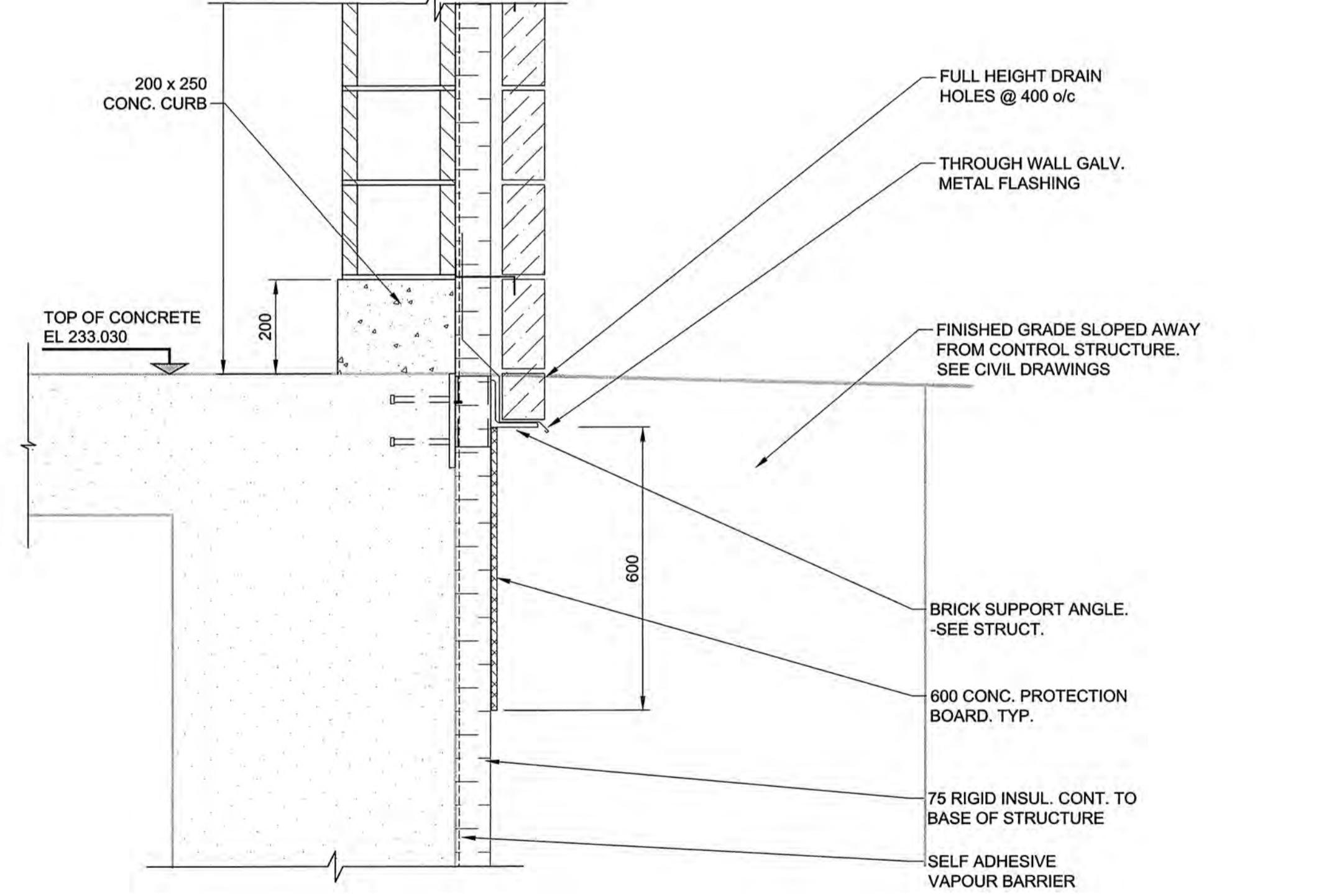
1 DETAIL Scale 1:10
