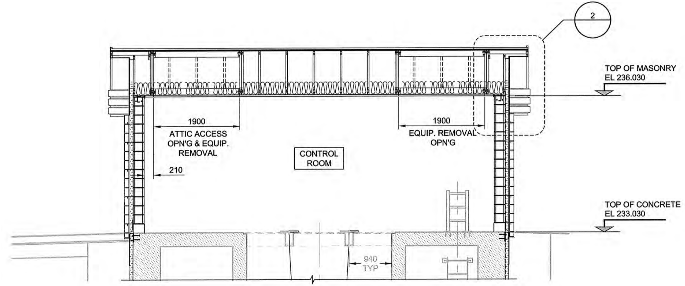
C SECTION LD-5848 Scale 1:50
